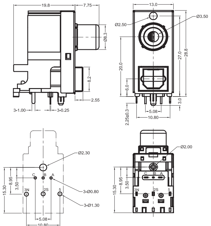
Recommended PCB Layout (Bottom View)
