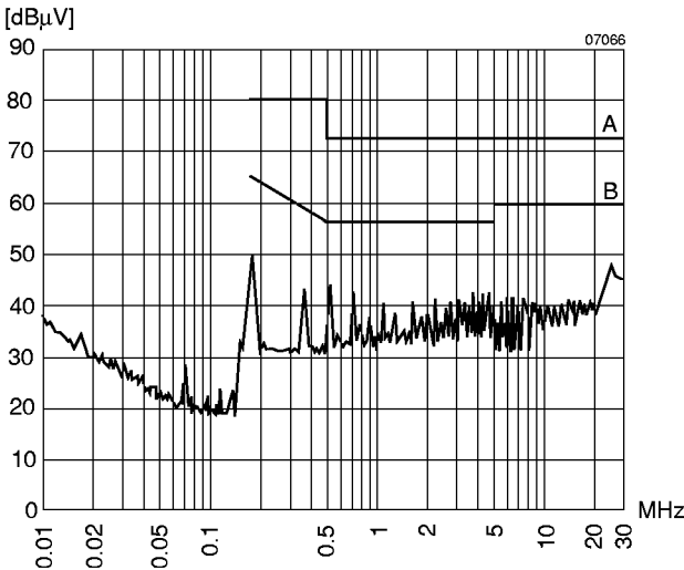
Fig. 6 Typical disturbance voltage (quasi-peak) at the input according to CISPR 11/22 and EN 55011/22, measured at U_{i\text{ rated}} and I_{o\text{ nom}} , e.g. for 24 IMR 25-05-2.
