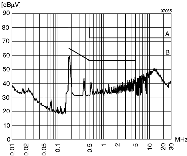
Fig. 5 Typical disturbance voltage (quasi-peak) at the input according to CISPR 11/22 and EN 55011/22, measured at U_{i\text{ rated}} and I_{o\text{ nom}} , e.g. for 12 IMR 25-05-2.
