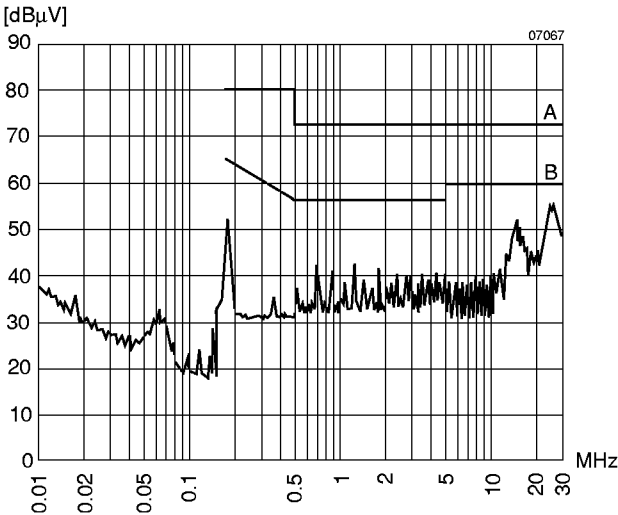
Fig. 7 Typical disturbance voltage (quasi-peak) at the input according to CISPR 11/22 and EN 55011/22, measured at U_{i rated} and I_{o nom} , e.g. for 48 IMR 25-05-2.
