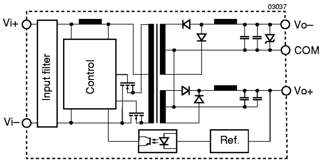
Fig. 2 Dual output converter block diagram
