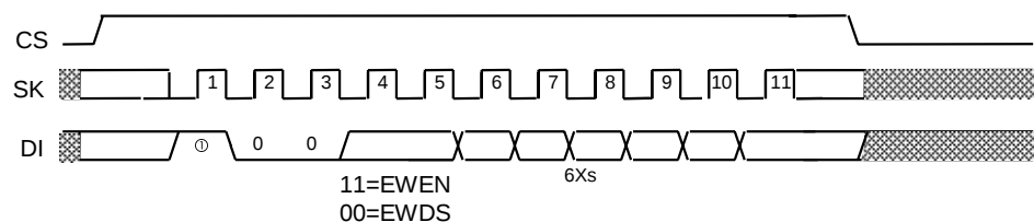
Figure 15 EWEN/EWDS Timing (S-29U330A)
