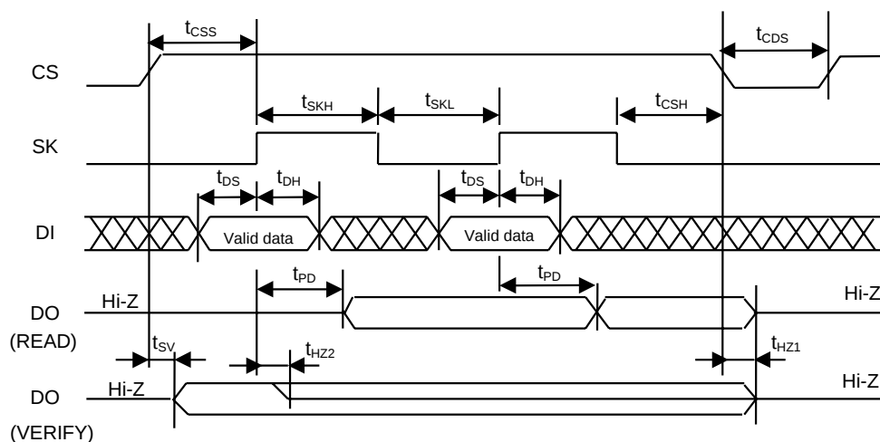
Figure 3 Timing Chart
