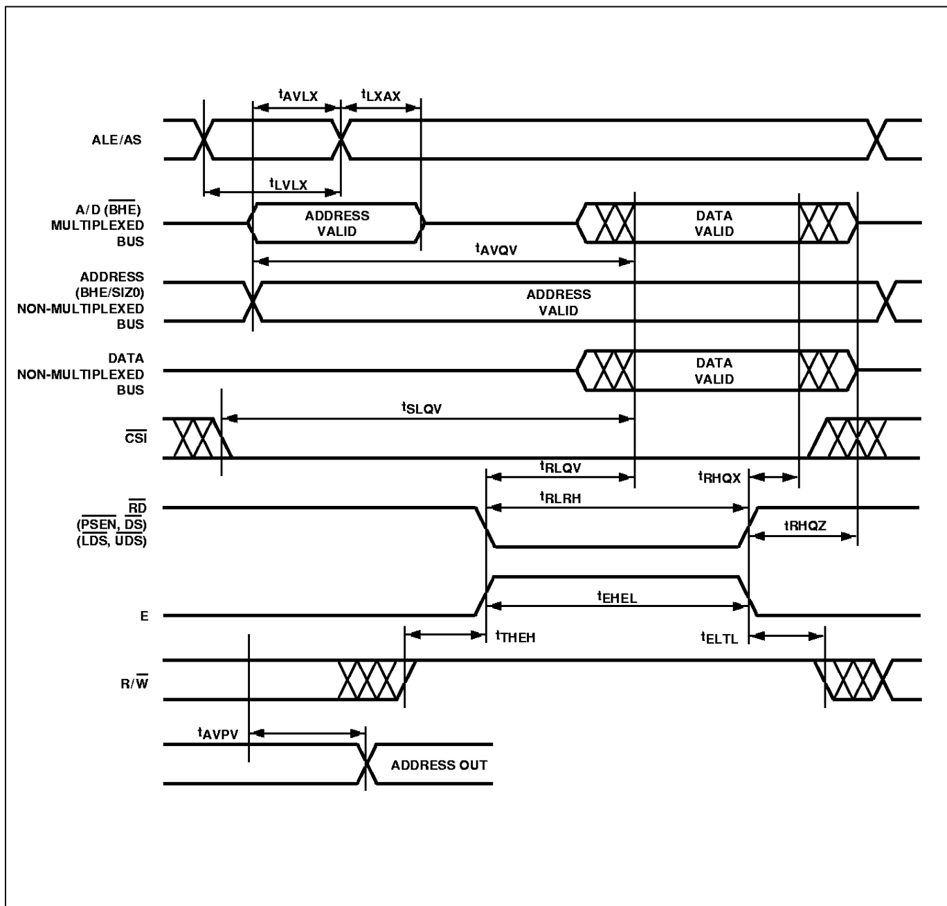
Figure 38. Read Timing
