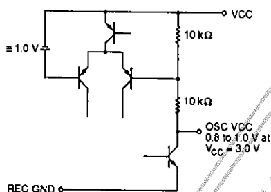
Figure 2. Oscillator supply
