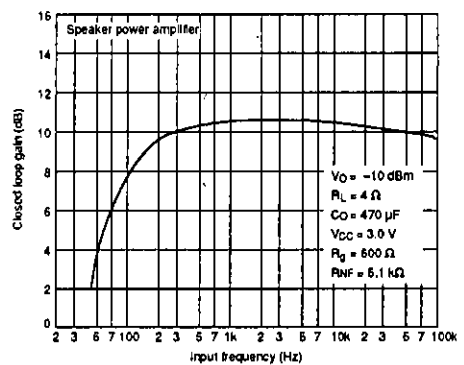
Closed-loop voltage gain vs. frequency (2)
