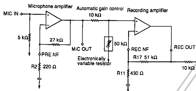
Figure 8. Microphone amplifier
