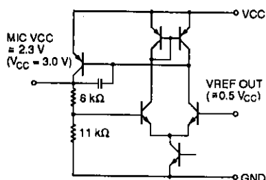
Figure 1. Microphone supply
