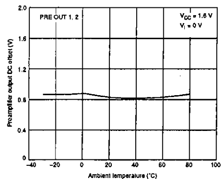
Output DC offset vs. ambient temperature (1)
