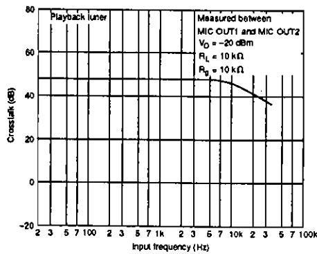
Crosstalk between channels vs. frequency (1)
