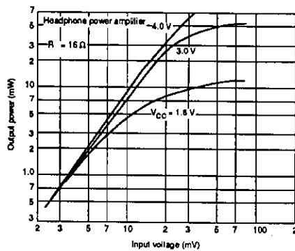
Output power vs. Input voltage
