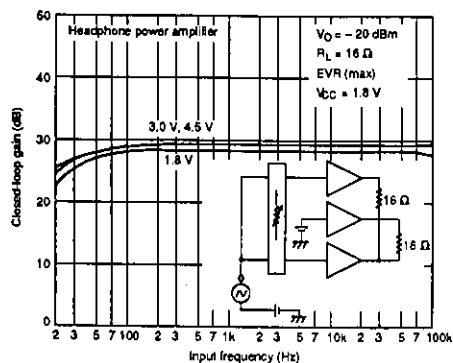
Closed-loop voltage gain vs. frequency (2)
