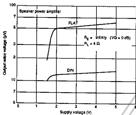
Output noise voltage vs. supply voltage (1)
