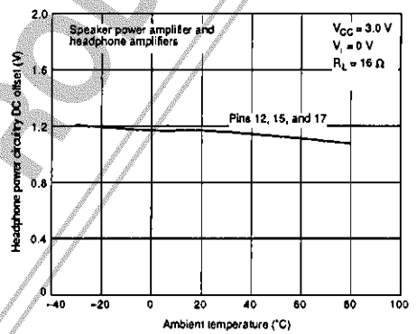
Amplifier DC offset vs. ambient temperature (6)
