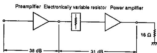
Figure 5. Preamplifier gain
