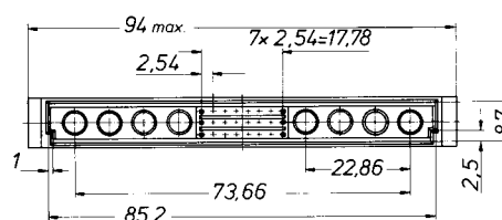
28 + 6* -poliq / contacts / contacts / contatti
