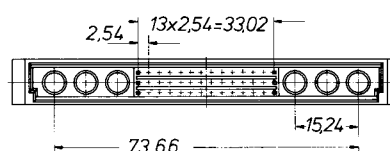
40 + 4* -poliq / contacts / contacts / contatti
