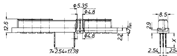
24 + 8* -polig / contacts / contacts / contatti
