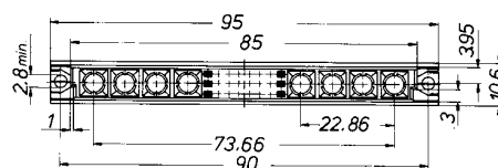
42 + 6* -polig / contacts / contacts / contatti
