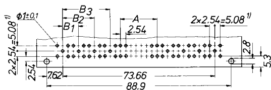
Lochbild / Printed circuit layout / Perçage du circuit imprimé / Dima foratura del circuito stampato
