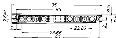
28 + 6* -polig / contacts / contacts / contatti
