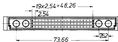
52 + 2* -poliq / contacts / contacts / contatti
