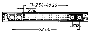
52 + 2* -polig / contacts / contacts / contatti
