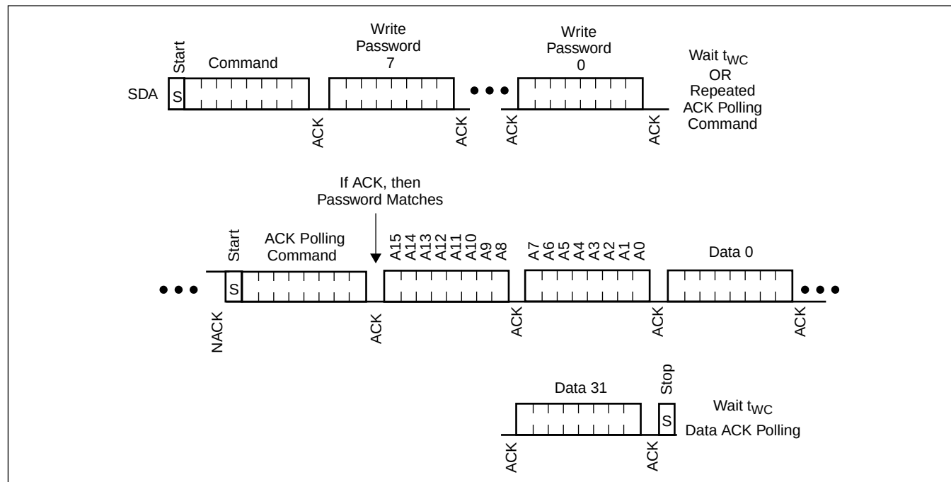
Figure 4. Sector Programming
