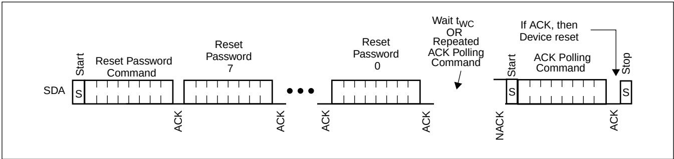
Figure 10. Reset Device
