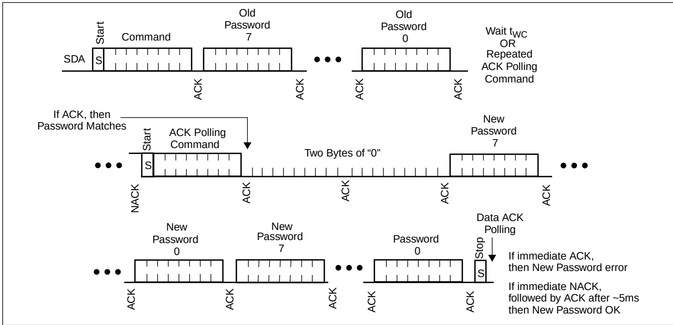
Figure 8. Change Passwords
