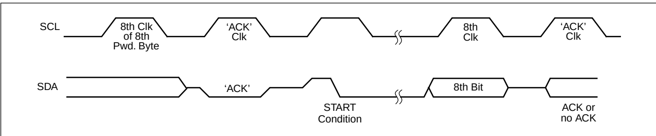
Figure 5. Acknowledge Polling
