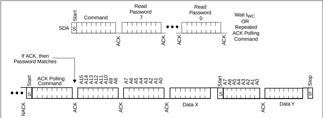
Figure 6. Random Read
