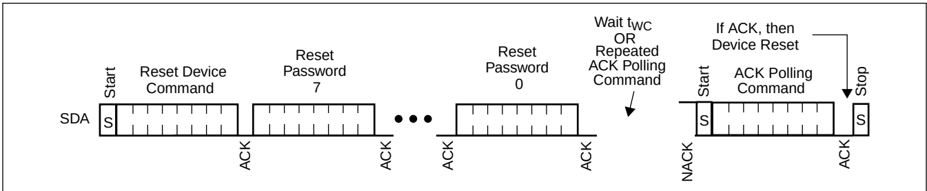
Figure 10. Reset Device
