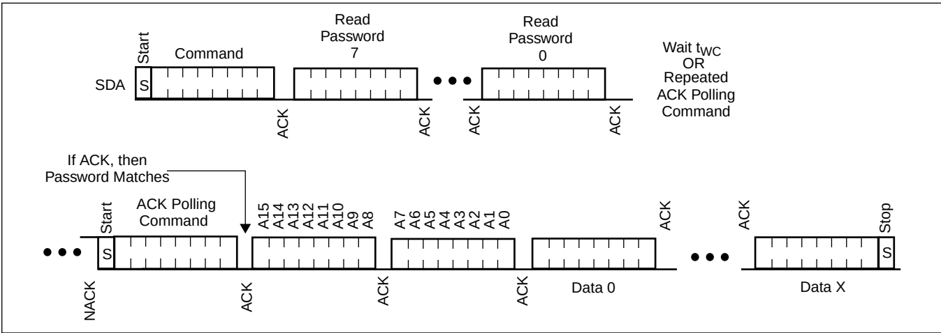
Figure 7. Sequential Read
