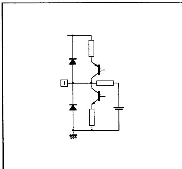
Figure 3 : CVBS Output
