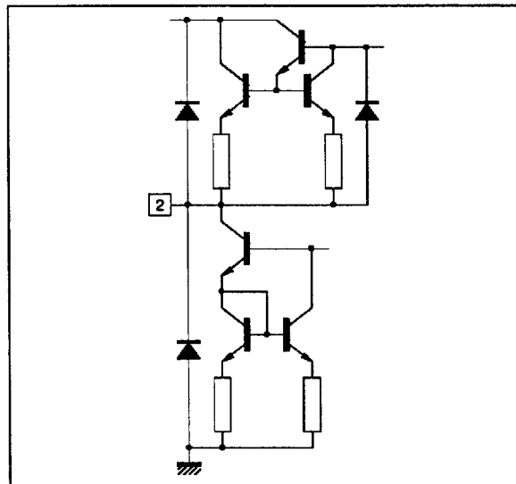
Figure 4 : Switching Input Standard + INT/EXT
