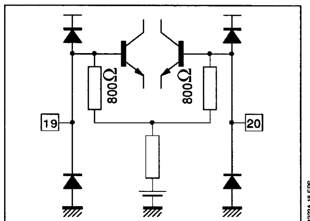
Figure 18 : Tuner AGC Output
