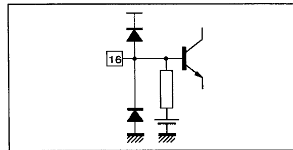
Figure 14 : External Audio Input
