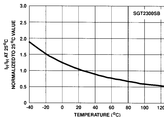
FIGURE 4. TYPICAL HOLDING CURRENT vs JUNCTION TEMPERATURE
