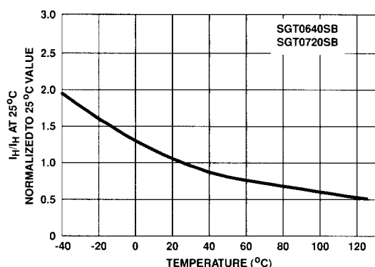
FIGURE 3. TYPICAL HOLDING CURRENT vs JUNCTION TEMPERATURE
