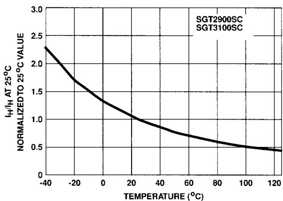
FIGURE 9. TYPICAL HOLDING CURRENT vs JUNCTION TEMPERATURE
