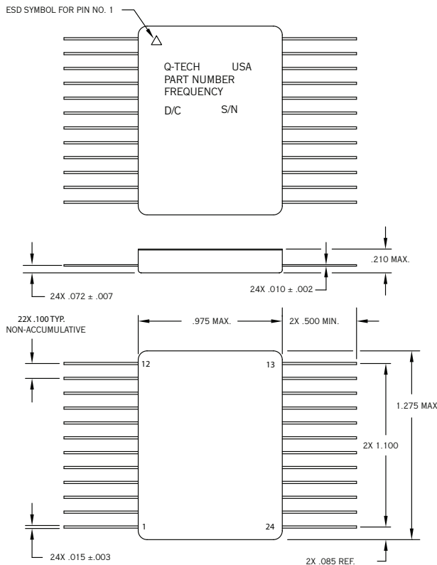
FIGURE 1 INTERFACE CONTROL DRAWING 24 pin Flat-Pack
