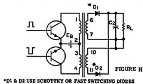
SCHEMATIC FOR SIZES 5 & 6 USING TRANSFORMERS AS LINEAR SWITCHING.
