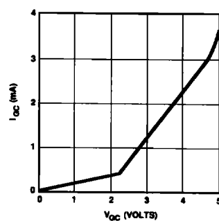
Figure 6. IVA-14228 I_{GG} vs. V_{GG} ; V_{CC} = 6\text{ V} , T_{\text{case}} = 25^\circ\text{C} .
