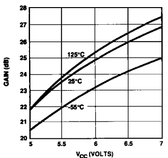
Figure 16. IVA-14228 Gain vs. V_{CC} and Temperature; V_{GC} = 0\text{ V} , Frequency = 1 GHz.
