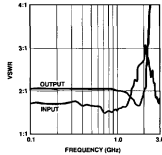
Figure 22. IVA-14208 VSWR vs. Frequency; V_{CC} = 6\text{ V} , V_{GG} = 0\text{ V} , T_{\text{case}} = 25^\circ\text{C} .
