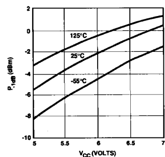
Figure 17. IVA-14228 P_{1dB} vs. V_{CC} and Temperature; V_{GC} = 0\text{ V} , Frequency = 1 GHz.
