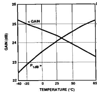
Figure 25. IVA-14208 Gain and P_{1\text{dB}} vs. Temperature; V_{CC} = 6\text{ V} , V_{GG} = 0\text{ V} , Frequency = 1 GHz.
