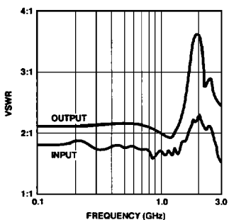
Figure 7. IVA-14228 VSWR vs. Frequency; V_{CC} = 6\text{ V} , V_{GG} = 0\text{ V} , T_{\text{case}} = 25^\circ\text{C} .
