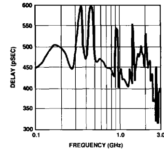
Figure 23. IVA-14208 Group Delay vs. Frequency; V_{CC} = 6\text{ V} , V_{GG} = 0\text{ V} , T_{\text{case}} = 25^\circ\text{C} .
