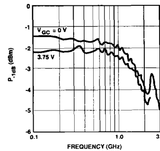
Figure 24. IVA-14208 P_{1\text{dB}} vs. Frequency and V_{GG} ; V_{CC} = 6\text{ V} , Frequency = 1 GHz, T_{\text{case}} = 25^\circ\text{C} .
