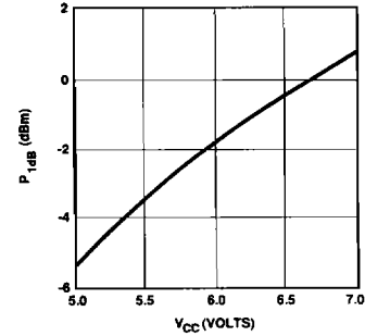
Figure 29. IVA-14208 P 1dB vs. V CC ; V GC = 0 V, Frequency = 1 GHz, T case = 25°C.
