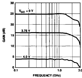
Figure 18. IVA-14208 Gain vs. Frequency and V_{GG} ; V_{CC} = 6\text{ V} , T_{\text{case}} = 25^\circ\text{C} .
