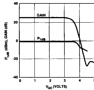
Figure 19. IVA-14208 Gain and P_{1\text{dB}} vs. V_{GG} ; V_{CC} = 6\text{ V} , Frequency = 1 GHz, T_{\text{case}} = 25^\circ\text{C} .
