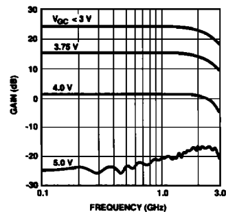
Figure 3. IVA-14228 Gain vs. Frequency and V_{GG} ; V_{CC} = 6\text{ V} , T_{\text{case}} = 25^\circ\text{C} .
