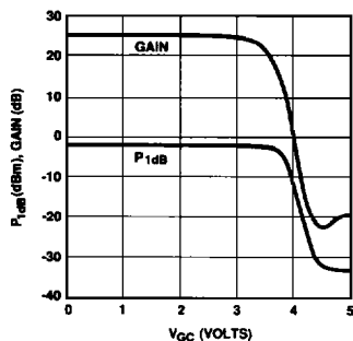
Figure 4. IVA-14228 P_{1\text{dB}} and Gain vs. V_{GG} ; V_{CC} = 6\text{ V} , T_{\text{case}} = 25^\circ\text{C} .
