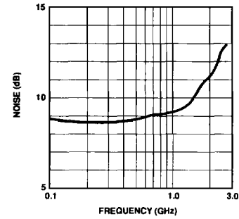
Figure 20. IVA-14208 Noise Figure vs. Frequency; V_{CC} = 6\text{ V} , V_{GG} = 0\text{ V} , T_{\text{case}} = 25^\circ\text{C} .
