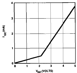
Figure 21. IVA-14208 I_{GG} vs. V_{GG} ; V_{CC} = 6\text{ V} , T_{\text{case}} = 25^\circ\text{C} .
