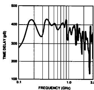
Figure 9. IVA-14228 Group Delay vs. Frequency; V_{GG} = 0\text{ V} , V_{CC} = 6\text{ V} , T_{\text{case}} = 25^\circ\text{C} .
