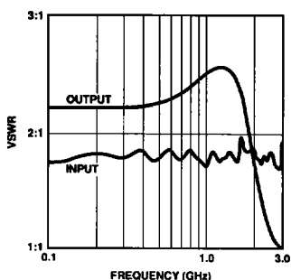
Figure 8. IVA-14228 VSWR vs. Frequency; V_{CC} = 6\text{ V} , V_{GG} = 5\text{ V} , T_{\text{case}} = 25^\circ\text{C} .
