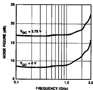
Figure 5. IVA-14228 Noise Figure vs. Frequency and V_{GG} ; V_{CC} = 6\text{ V} , T_{\text{case}} = 25^\circ\text{C} .
