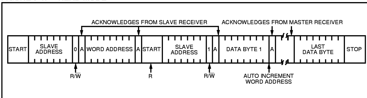
FIGURE 8-1: READ MODE
