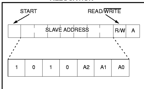
FIGURE 4-1: SLAVE ADDRESS ALLOCATION
