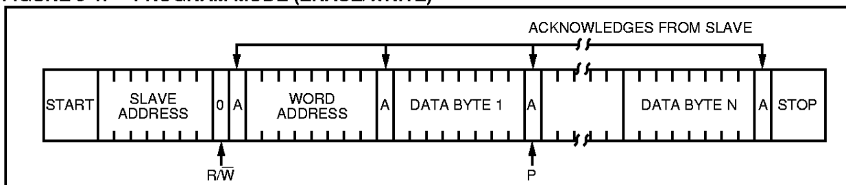
FIGURE 6-1: PROGRAM MODE (ERASE/WRITE)
