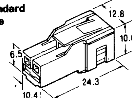
Double Lock Type
