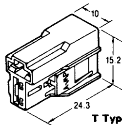
Parallel Type
