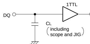
Fig.1 Output load
