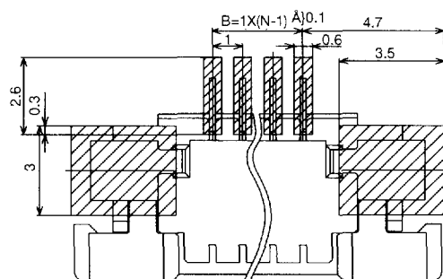
MOUNTING LAYOUT
