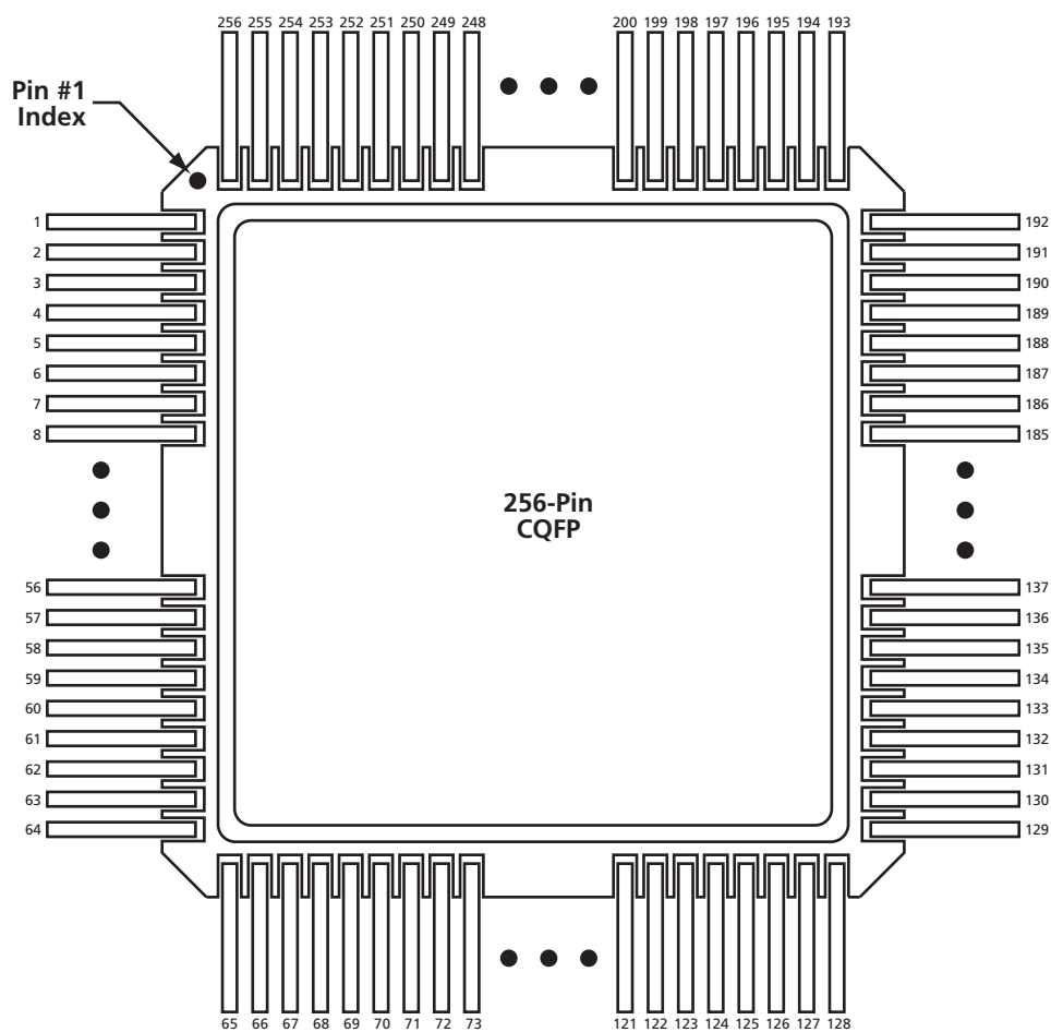
Figure 2-5 • 256-Pin CQFP (Top View)
