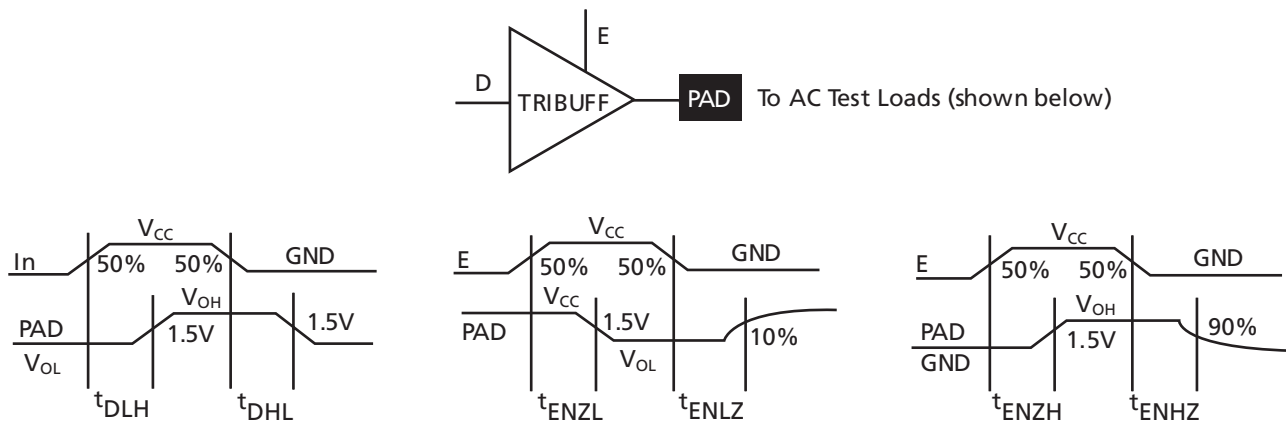
Figure 1-9 • Output Buffer Delays
