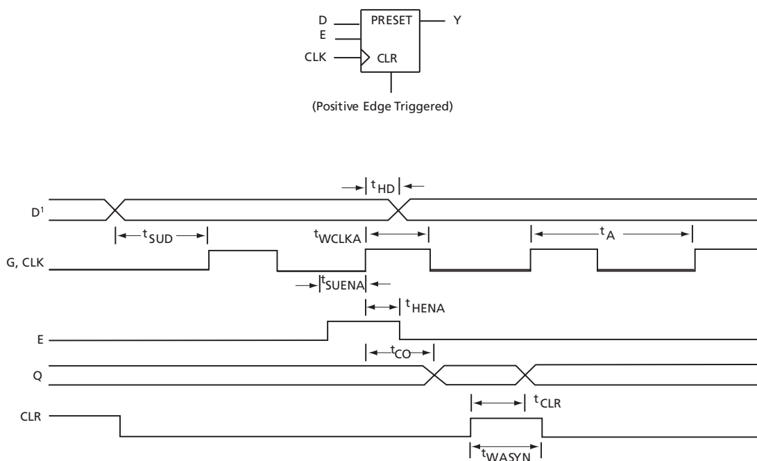
Figure 1-13 • Flip-Flops and Latches (RT1280A, A1280A)
