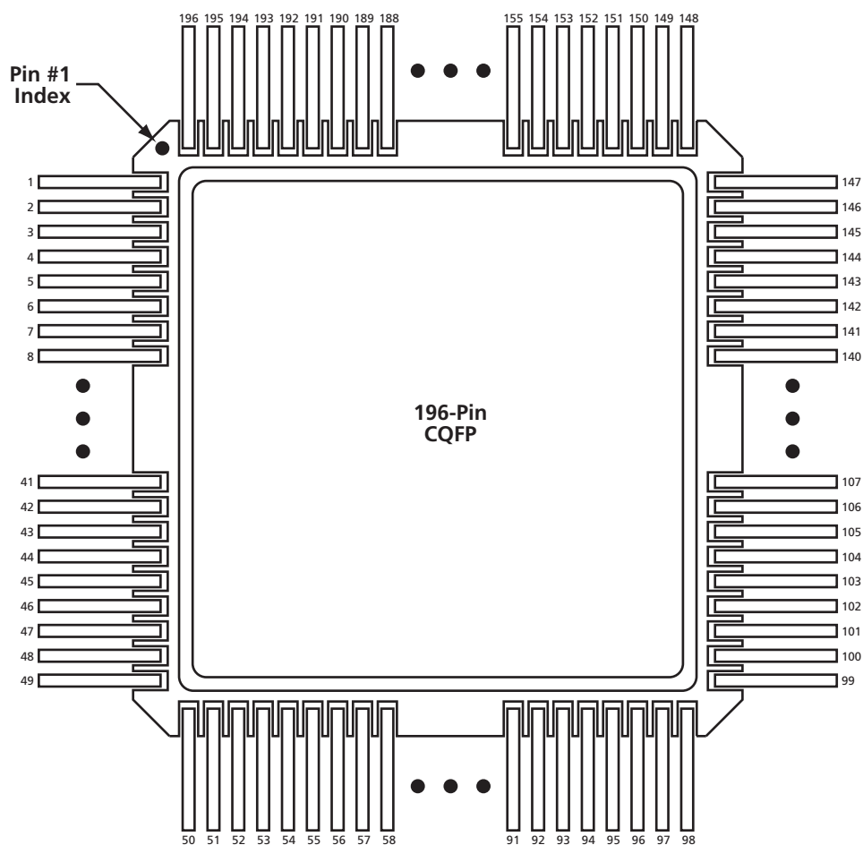
Figure 2-4 • 196-Pin CQFP (Top View)
