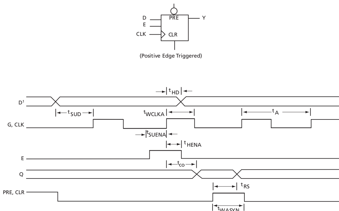
Figure 1-13 • Flip-Flops and Latches (RT1280A, A1280A)
