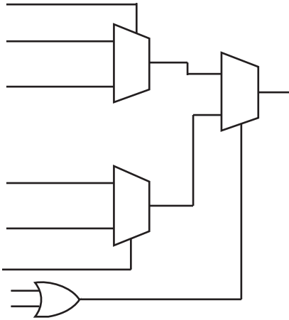
Figure 1-3 • RT1020 Logic Module
