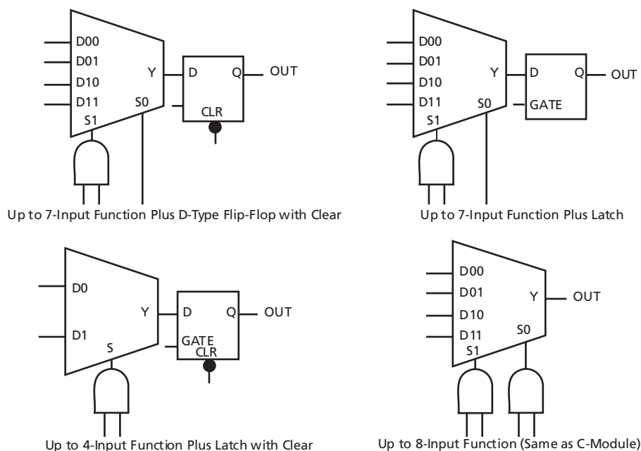
Figure 1-2 • S-Module Implementation
