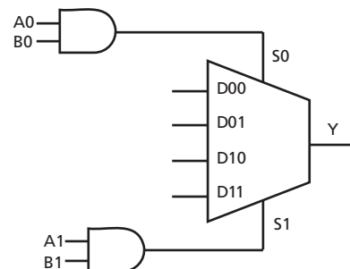
Figure 1-1 • C-Module Implementation
