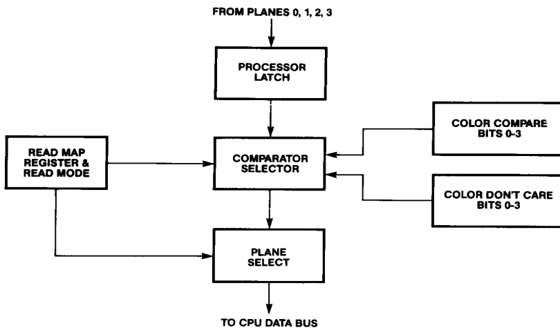
Figure 3. 82C431 Read Process
