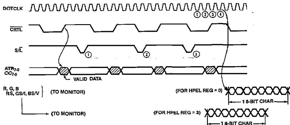
Figure 12. Alphanumeric Data Timings
