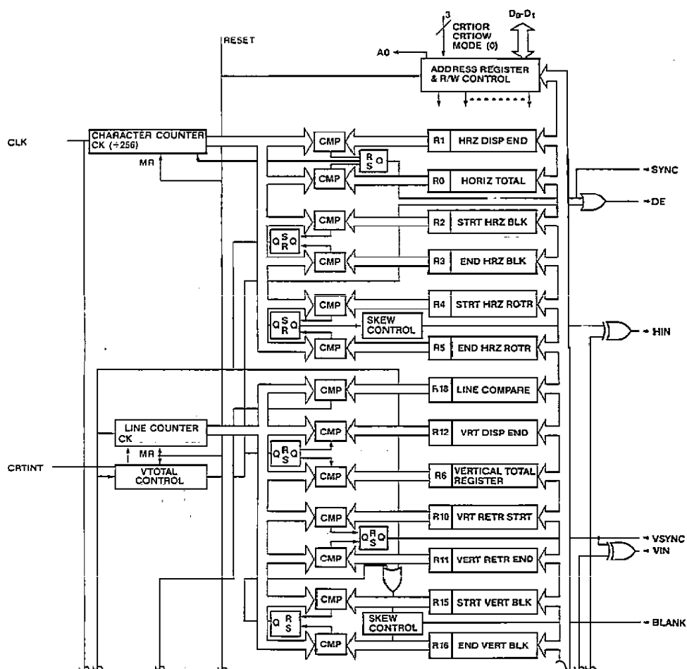
Figure 14. 82C434A Function Diagram
