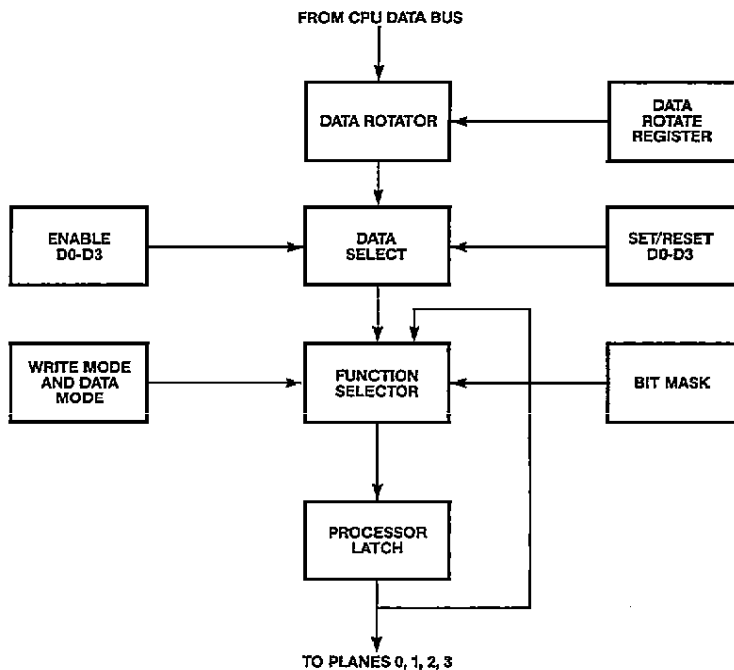
Figure 2. 82C431 Write Process
