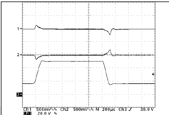
Figure 19: Output voltage response to step-change in input voltage (16V - 50V - 16V). Load cap: 10 \mu F, 100m \Omega ESR tantalum cap and 1 \mu F ceramic cap. Ch 1: +Vout (500mV/div); Ch 2: -Vout (500mV/div); Ch 3: Vin (20V/div).
