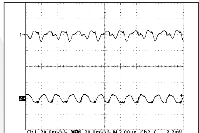
Figure 22: Output voltage ripple, +Vout (Ch 1) and -Vout (Ch 2), at nominal input voltage and full load current evenly split (20mV/div). Load capacitance: 1 \mu F ceramic cap and 10 \mu F tantalum cap. Bandwidth: 10MHz. See Figure 20.
