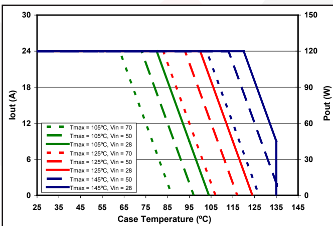
Figure 11: Total Output Current / Total Output Power derating curve as a function of T_{case} and the maximum desired power MOSFET junction temperature (see Note 15).
