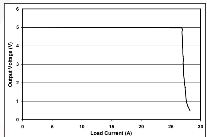
Figure 12: Positive output voltage vs. total load current, evenly split, showing typical current limit curves at V_{in} = 28V .
