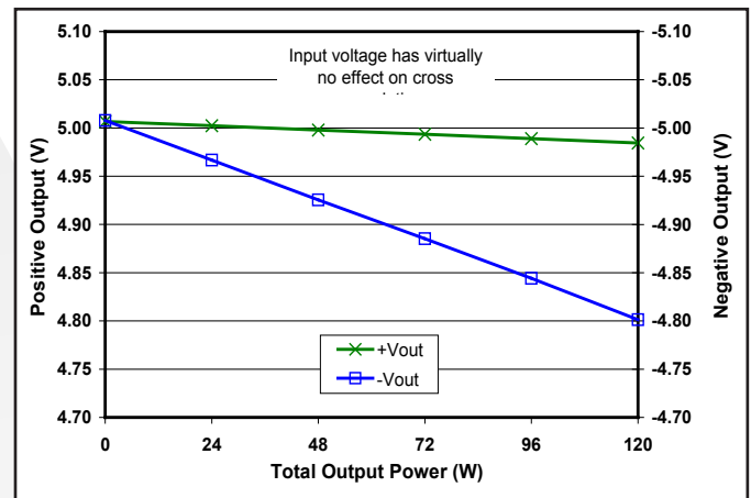
Figure 10: Load regulation vs. total output power from zero to to full load where -I out equals three times +I out at nominal input voltage and T_{case} = 25^{\circ}C .
