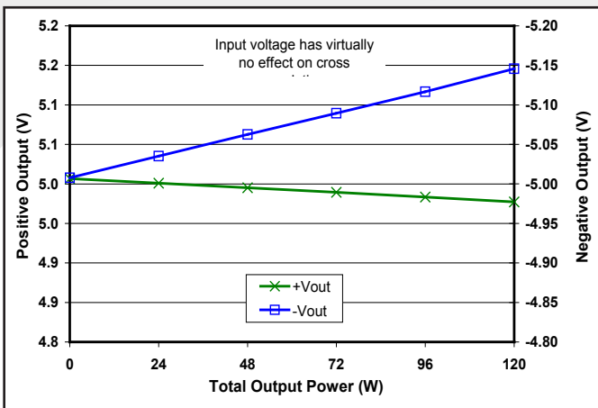
Figure 9: Load regulation vs. total output power from zero to to full load where +I out equals three times -I out at nominal input voltage and T_{case} = 25^{\circ}C .
