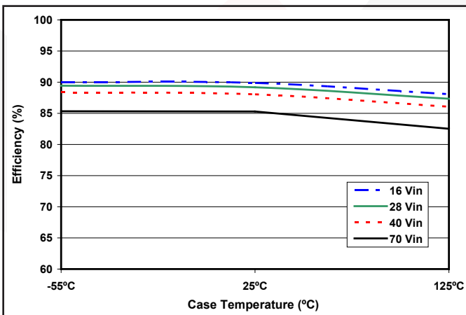
Figure 5: Efficiency at 60% load (7.2A load on +5V and 7.2A load on -5V) versus case temperature for V_{in} = 16V, 28V, 40V, and 70V .
