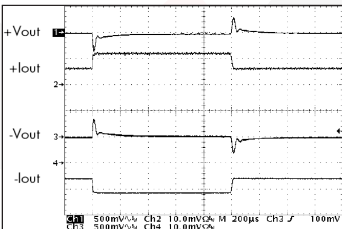
Figure 17: Output voltage response to step-change in total load current (50%-100%-50%) of total Iout (max) split 50%/50%. Load cap: 1 \mu F ceramic cap and 10 \mu F, 100m \Omega ESR tantalum cap. Ch 1: +Vout (500mV/div); Ch 2: +Iout (10A/div); Ch 3: -Vout (500mV/div); Ch 4: -Iout (10A/div).
