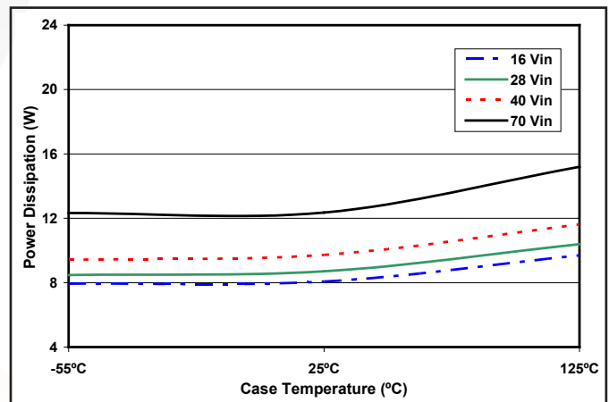
Figure 6: Power dissipation at 60% load (7.2A load on +5V and 7.2A load on -5V) versus case temperature for V_{in} = 16V, 28V, 40V, and 70V .
