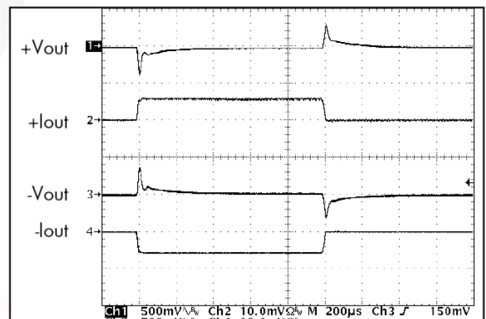
Figure 18: Output voltage response to step-change in total load current (0%-50%-0%) of total Iout (max) split 50%/50%. Load cap: 1 \mu F ceramic cap and 10 \mu F, 100m \Omega ESR tantalum cap. Ch 1: +Vout (500mV/div); Ch 2: +Iout (10A/div); Ch 3: -Vout (500mV/div); Ch 4: -Iout (10A/div).
