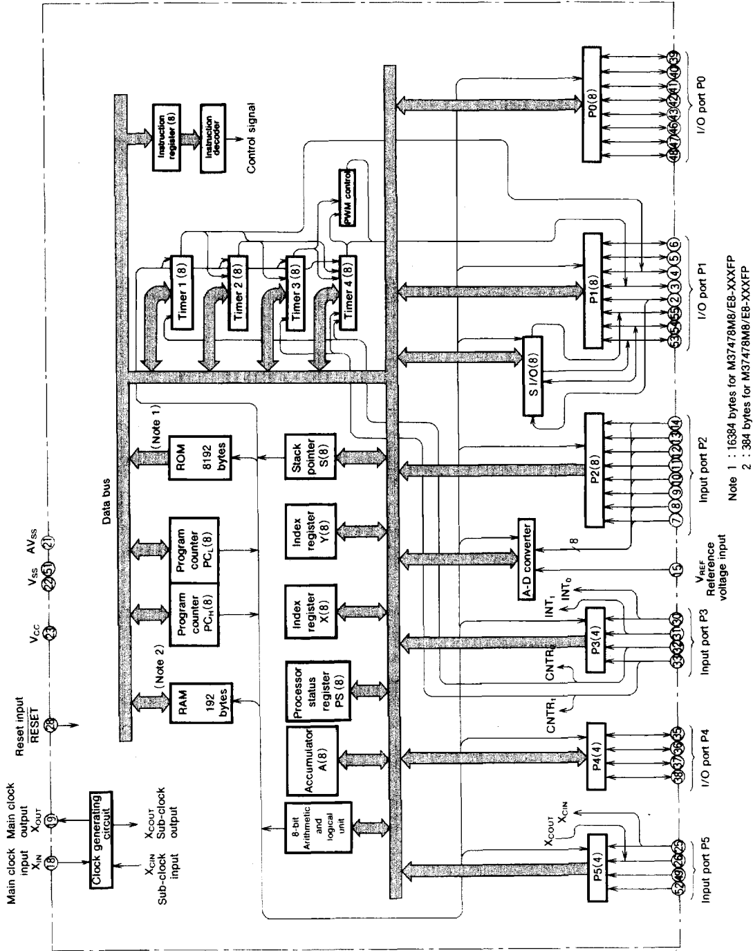
M37478M4-XXXXFP BLOCK DIAGRAM
