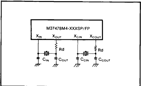
Fig. 24 Example of ceramic resonator circuit (7478 group)
