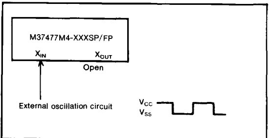
Fig. 25 External clock input circuit (7477 group)
