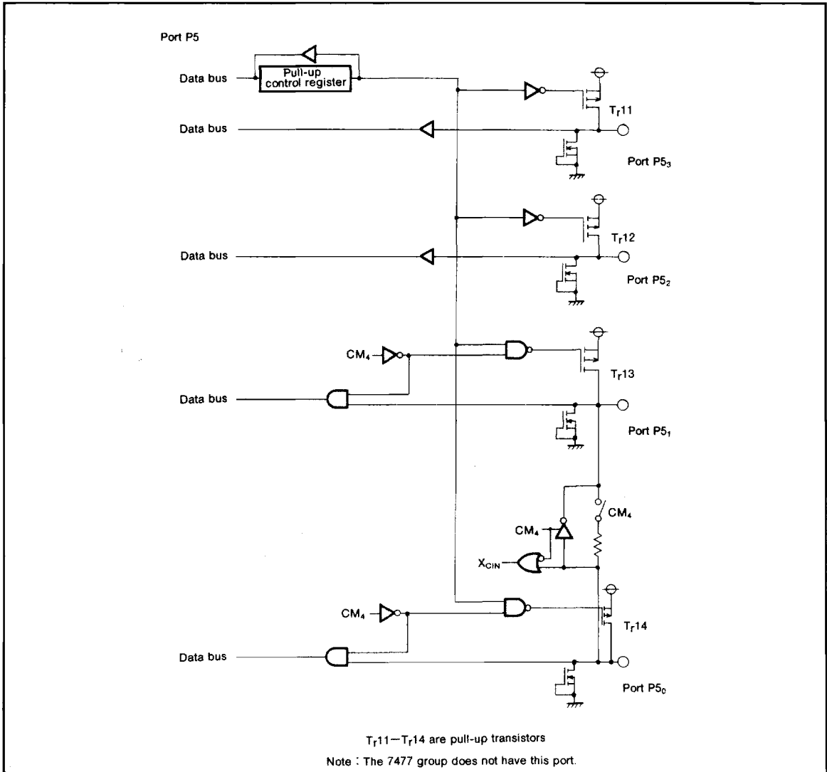
Fig. 22 Block diagram of port P5
