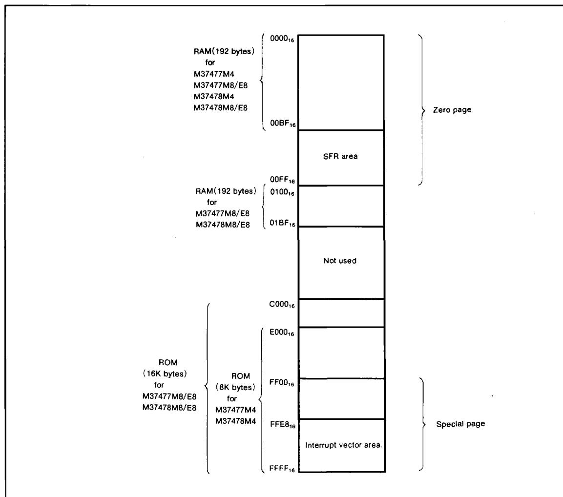
Fig. 2 Memory map
