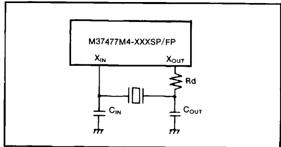
Fig. 23 Example of ceramic resonator circuit (7477 group)
