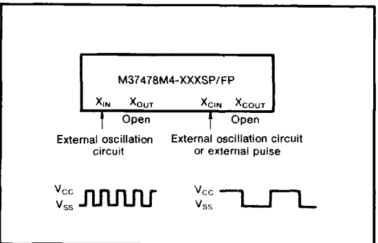
Fig. 26 External clock input circuit (7478 group)
