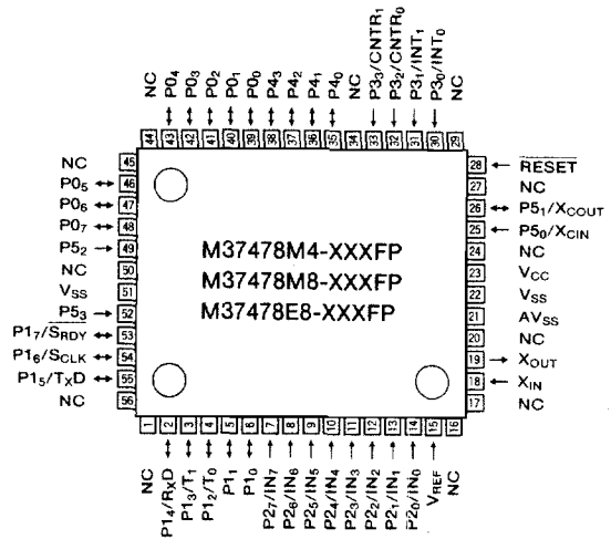
Outline 56P6N-A
