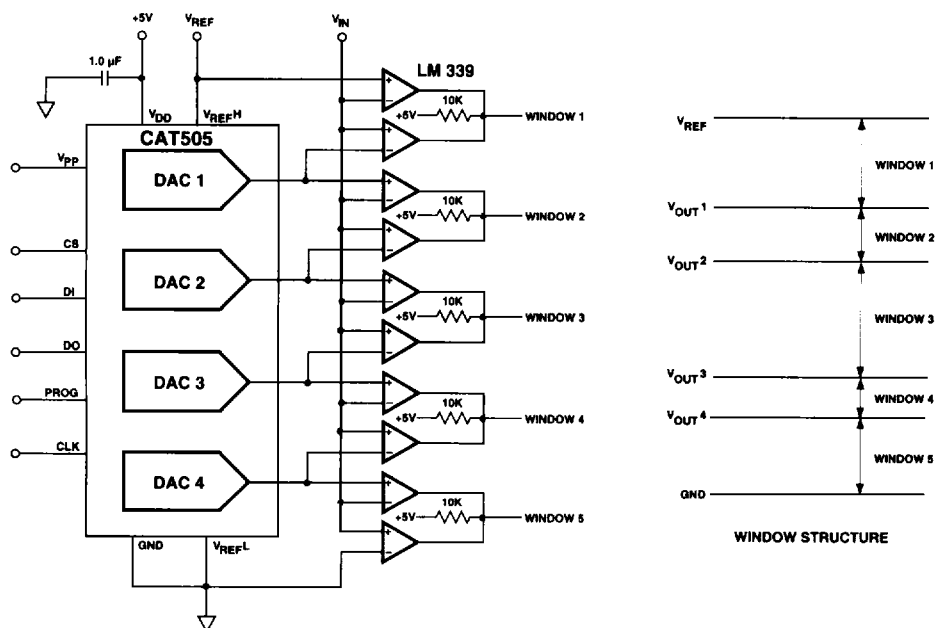
Staircase Window Comparator
