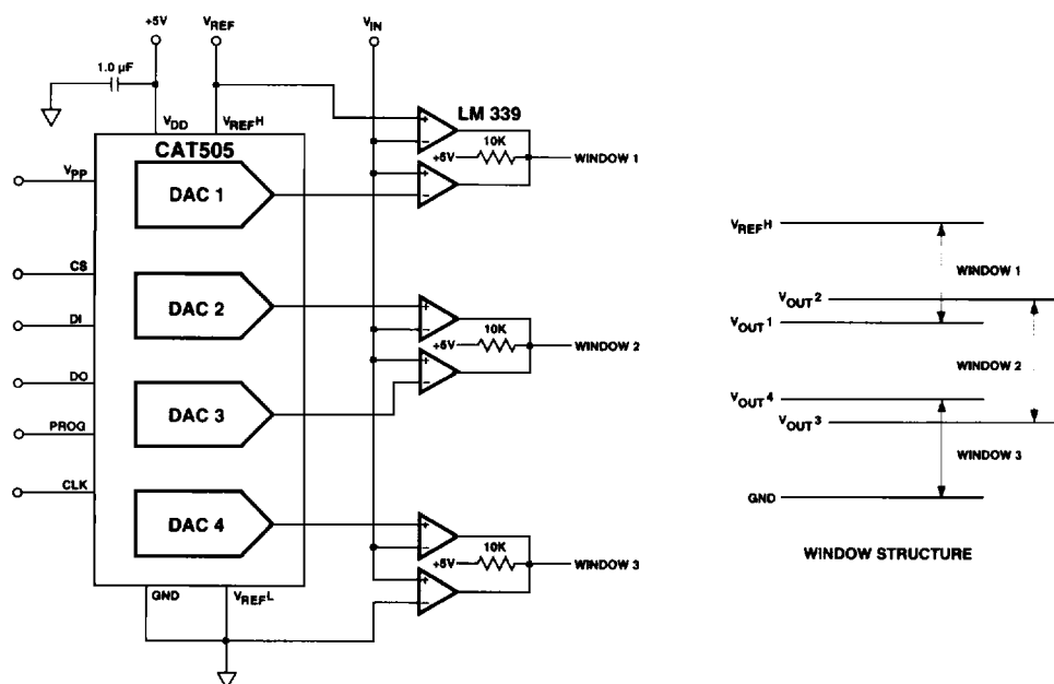
Overlapping Window Comparator
