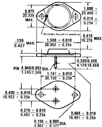
FIGURE 1 All dimensions in INCH m.m.
