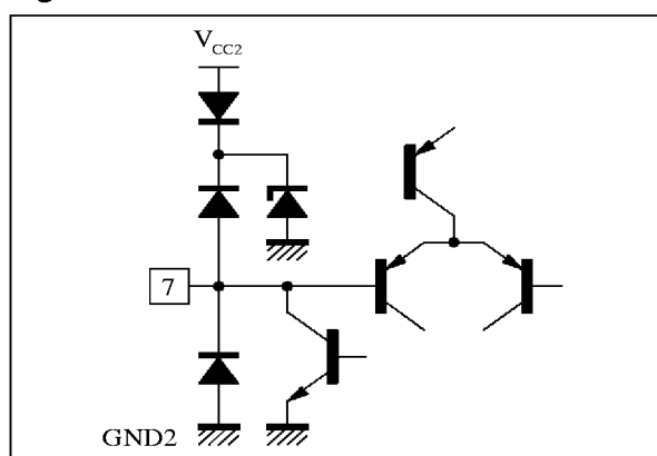
Figure 10 : Pin 7 - SCL
