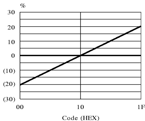
Figure 5 : Volume Control Curve
