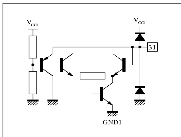
Figure 22 : Pin 31 - BCL
