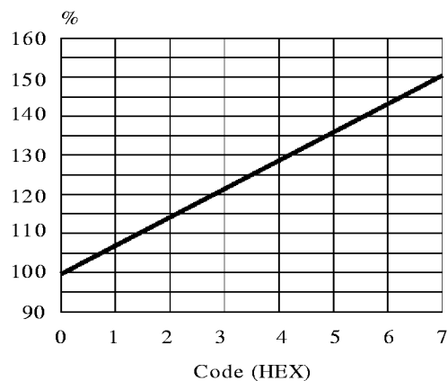
Figure 4 : Peaking Control (2T overshoot)
