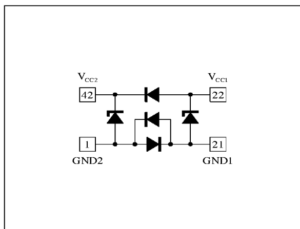
Figure 31 : Pins 42, 22 - V_{CC2} , V_{CC1}
