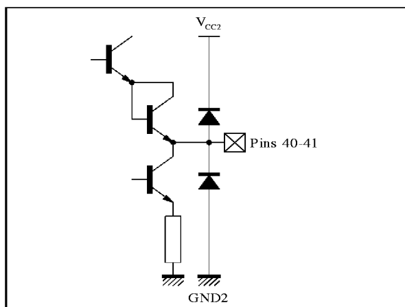
Figure 30 : Pins 40, 41 - RYO, BYO
