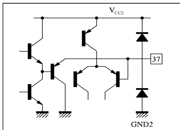
Figure 28 : Pin 37 - LFB/SC
