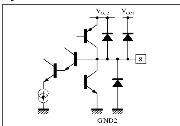
Figure 11 : Pin 8 - FTUN1
