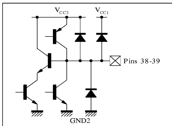
Figure 29 : Pins 38, 39 - BYI, RYI
