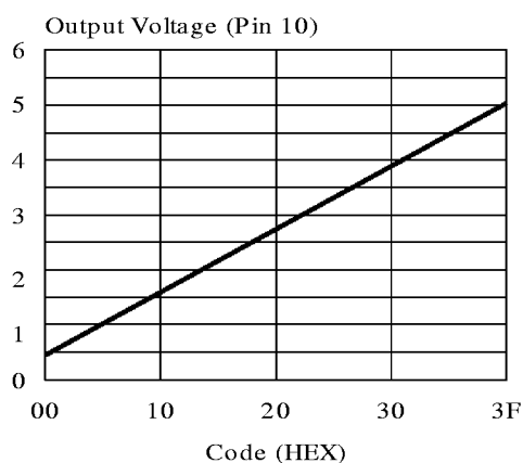
Figure 5 : Volume Control Curve
