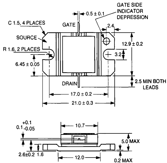
PACKAGE OUTLINE T-61
