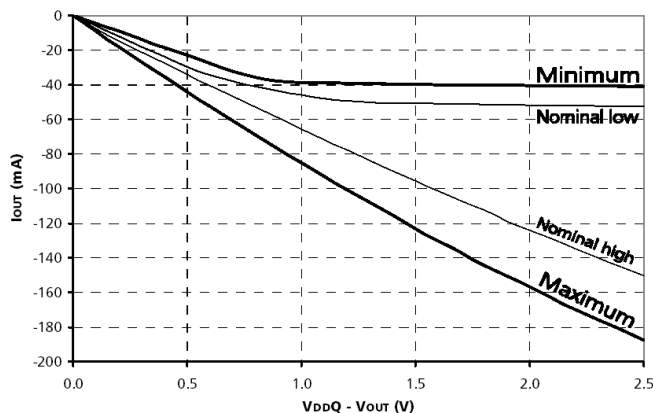
Figure 10: Pull-Up Characteristics
