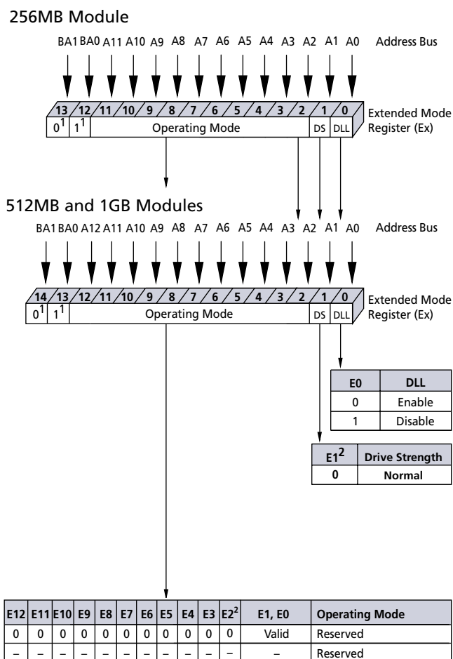
Figure 7: Extended Mode Register Definition Diagram
