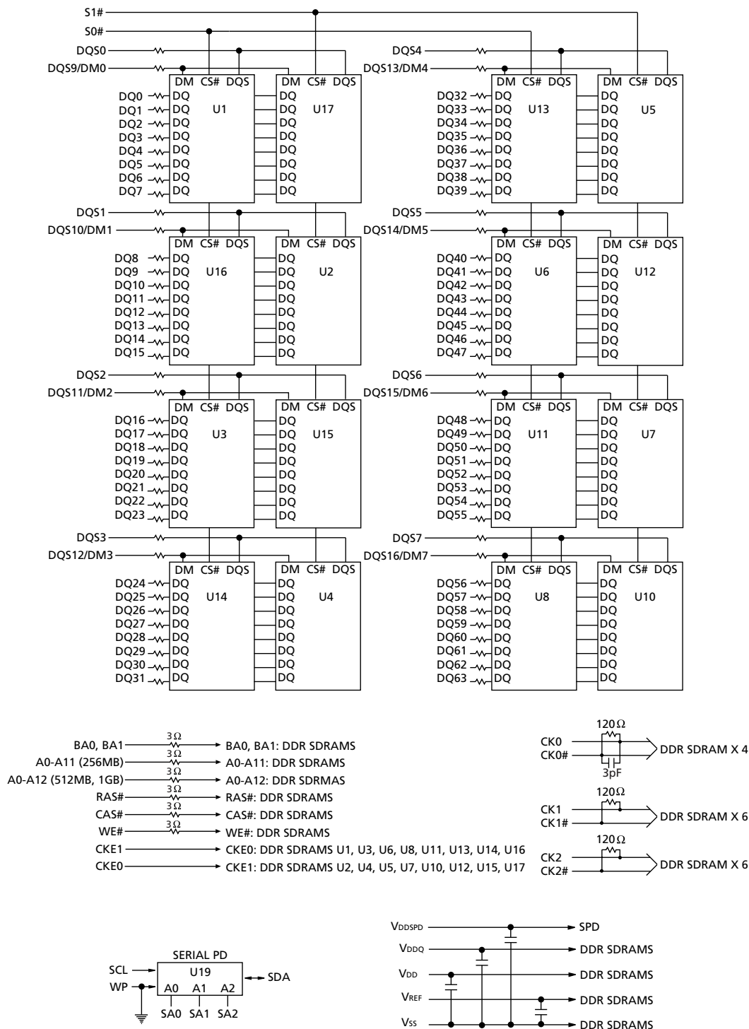
Figure 4: Functional Block Diagram -335 Speed Grade
