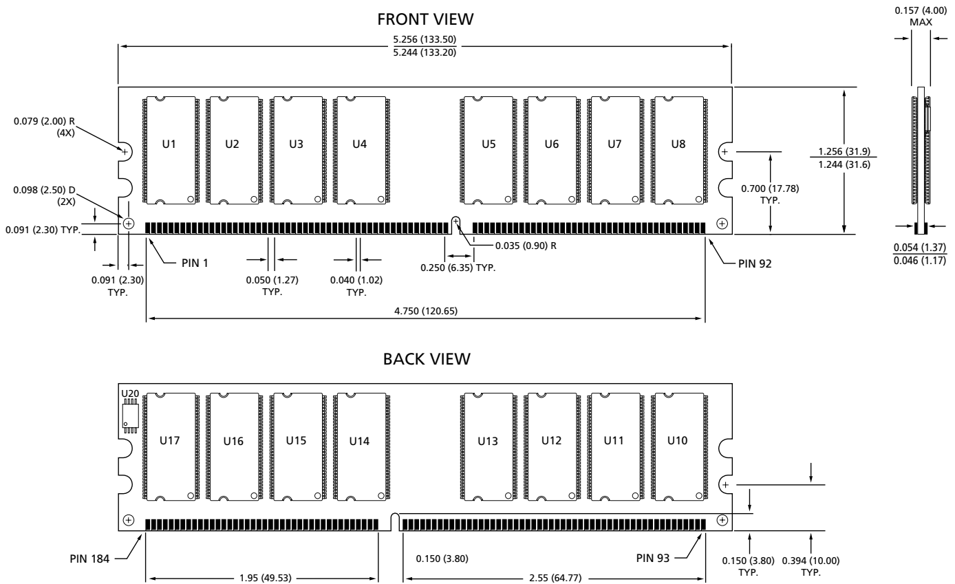
Figure 15: Standard 184-PIN DDR DIMM Dimensions, -202, -265, -26A, and -262 Speed Grades
