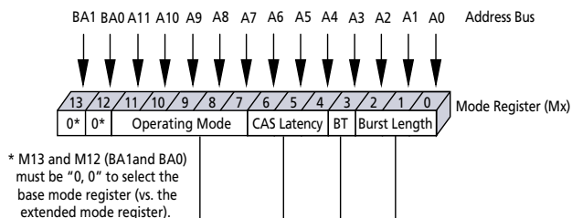
Figure 5: Mode Register Definition Diagram
