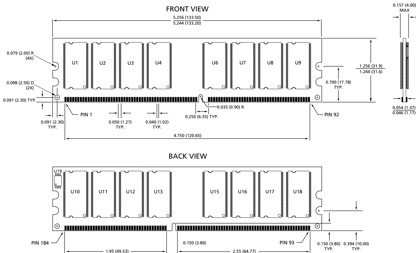
Figure 16: Standard 184-PIN DDR DIMM Dimensions, -335 Speed Grade
