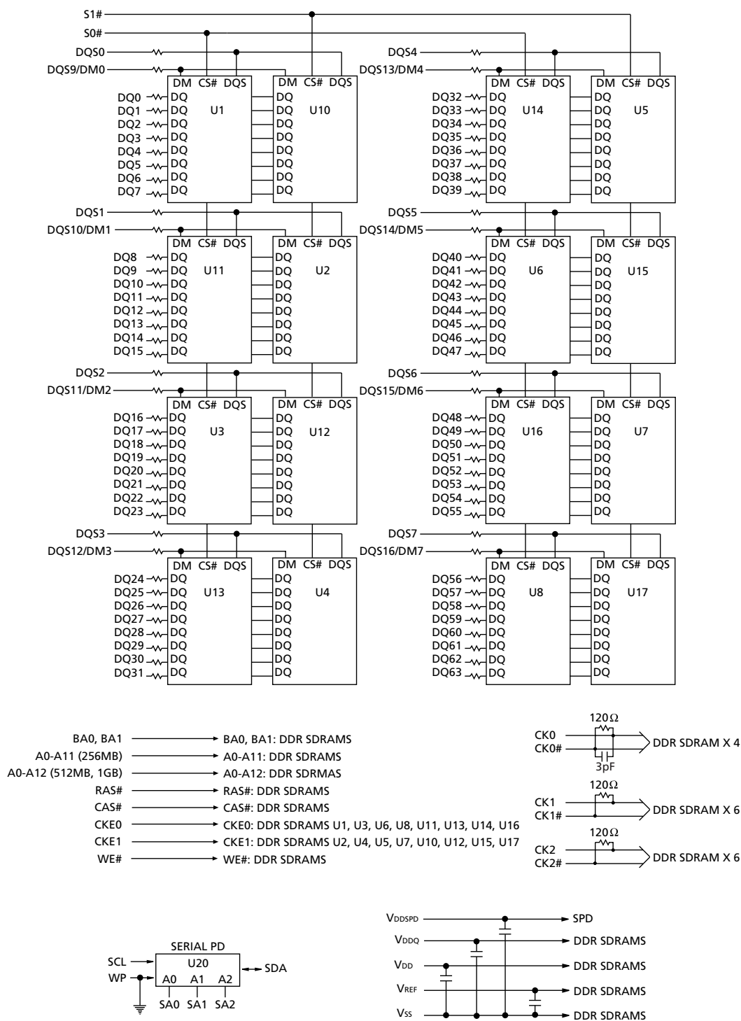
Figure 3: Functional Block Diagram -262, -26A, -265, and -202 Speed Grades
