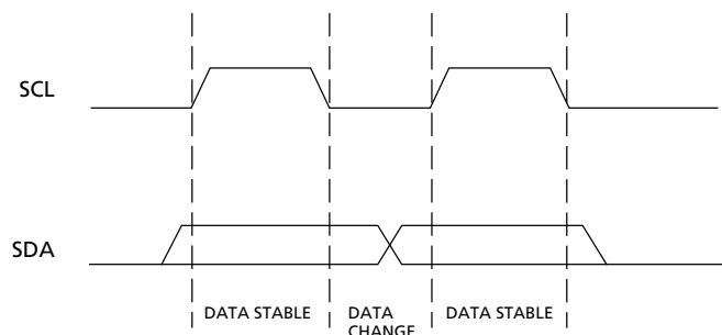
Figure 11: Data Validity
