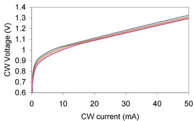
Typical IV curve at T c = 25°C, 45°C, 65°C and 85°C
