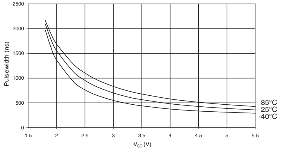
Figure 27-94. Minimum Reset Pulwidth vs. V_{CC}
