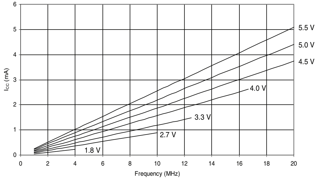
Figure 28-82. ATmega324P:Reset Supply Current vs Vcc 1-20MHz
