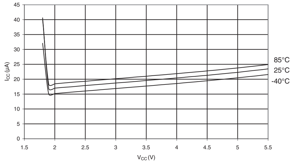
Figure 27-136. Brownout Detector Current vs. V_{CC}
