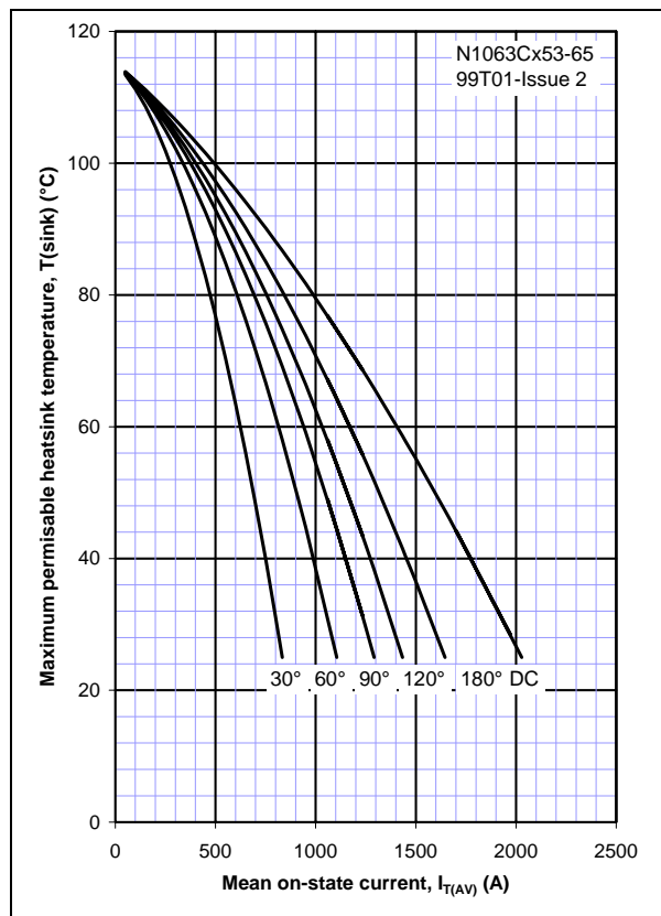
Figure 12, Heatsink temperature vs. mean current, squarewave, single side cooled
