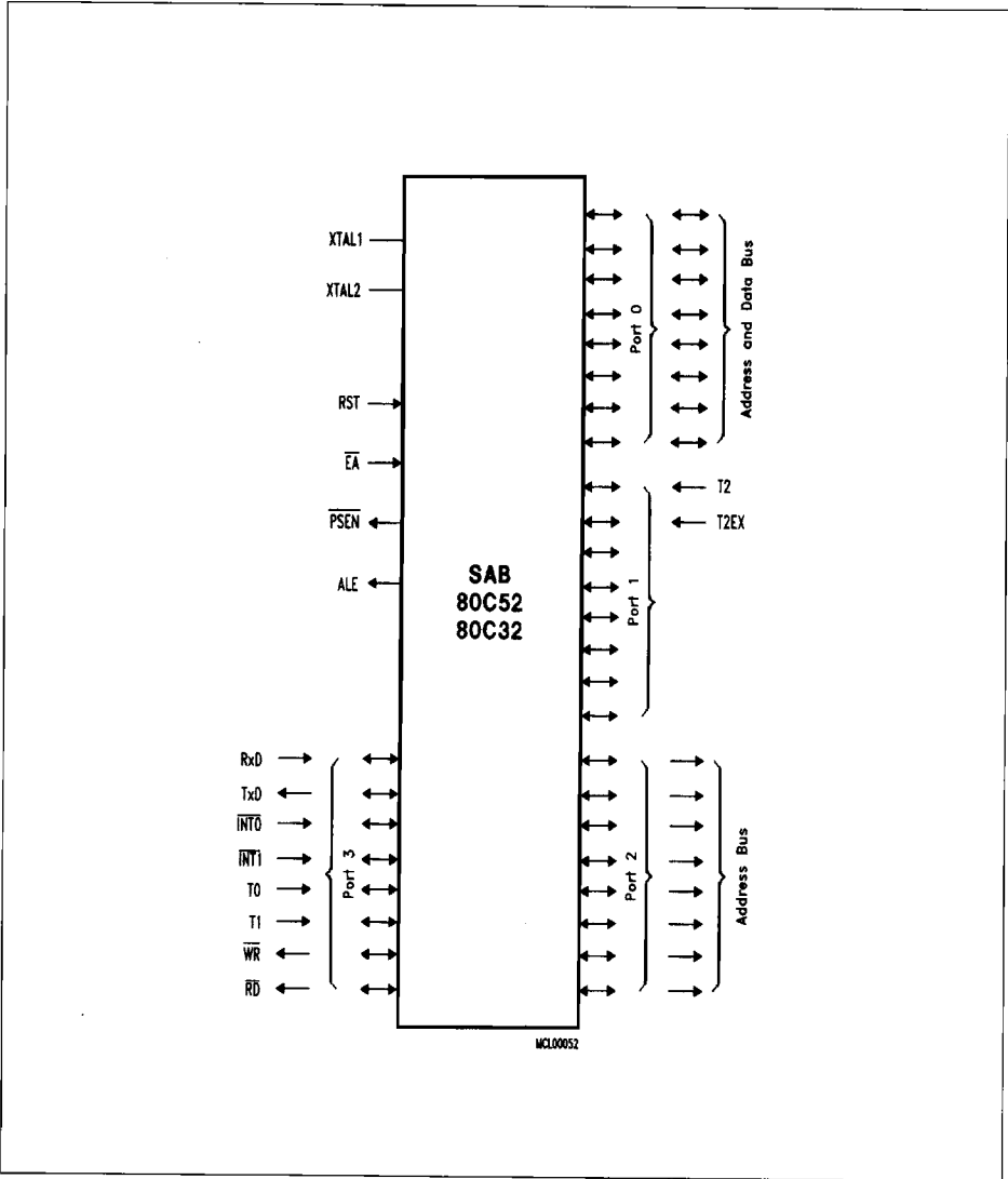
Logic Symbol
