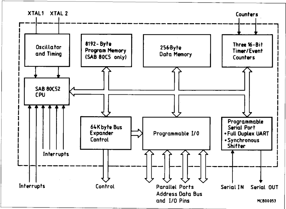
Figure 1 Block Diagram
