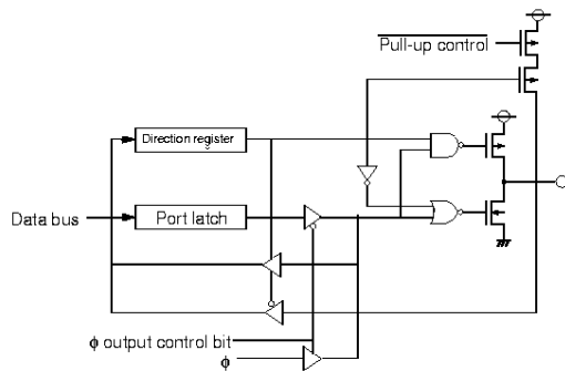
(5) Port P41
