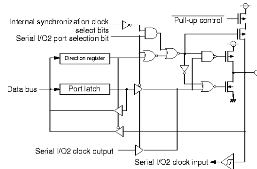
(12) Port P52
