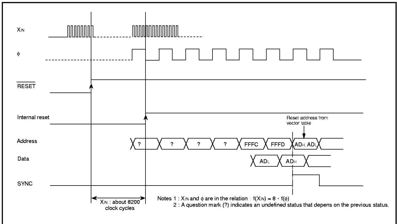
Fig. 34 Reset sequence
