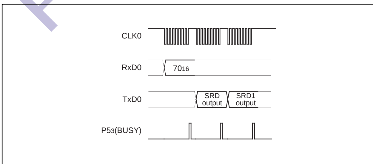
Figure DD-4. Timing for reading the status register
