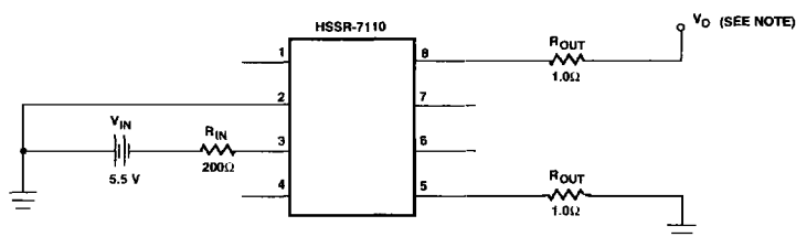
Figure 20. Burn-In Circuit.
