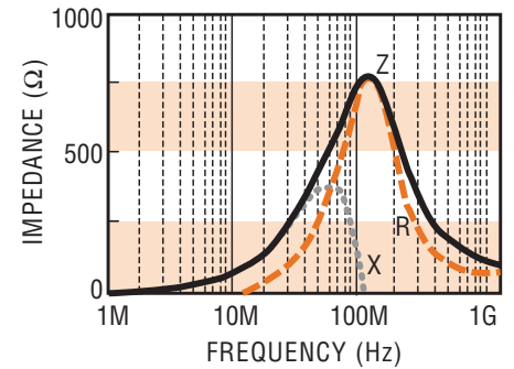
FBM1206-102 □
