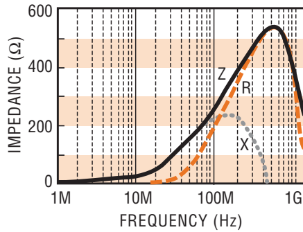
FBM0402-301 □
