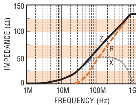
FBM0402-600 □
