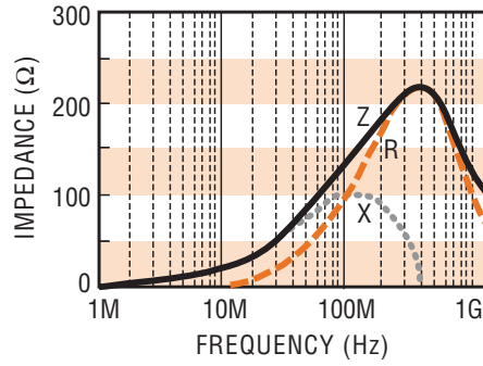
FBM0805-121 □
