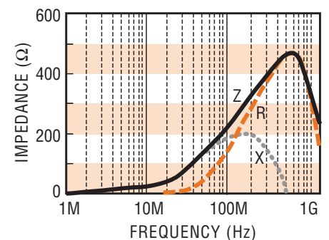
FBM0402-241 □
