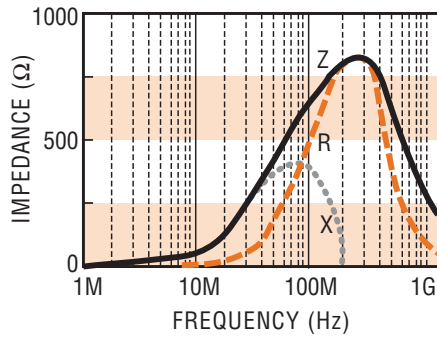
FBM0402-601 □
