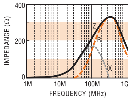
FBM1206-221 □
