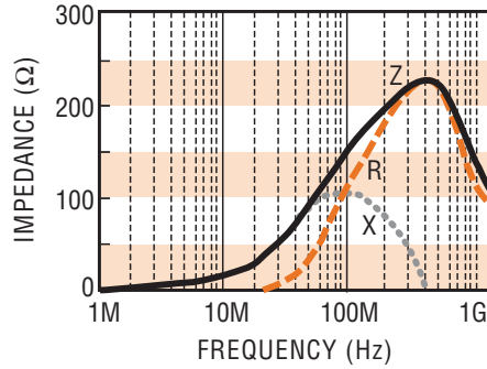
FBM1206-151 □
