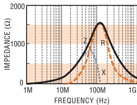
FBM0402-152 □
