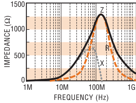
FBM0402-102 □
