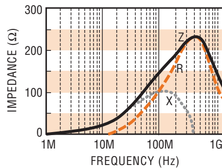
FBM0805-151 □
