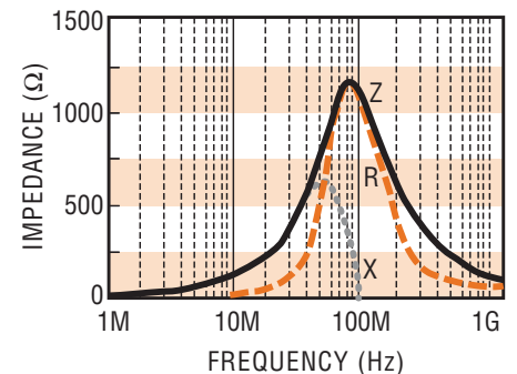
FBM1206-152 □
