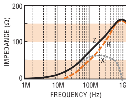
FBM0402-800 □
