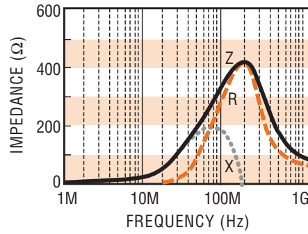
FBM1206-301 □
