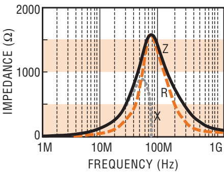
FBM0805-152 □
