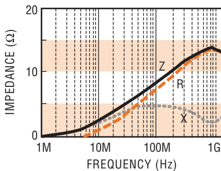
FBM0402-100 □
