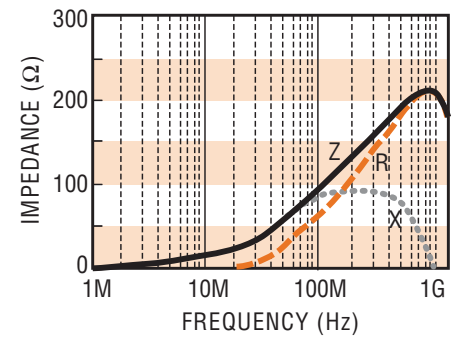
FBM0402-121 □
