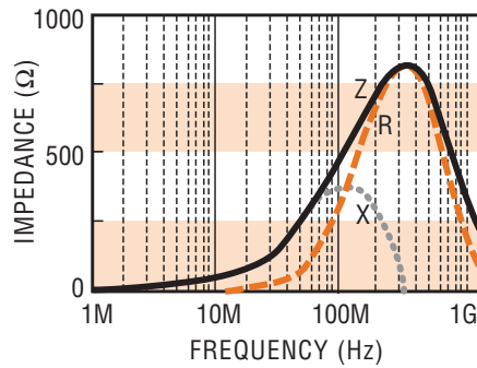
FBM0402-471 □
