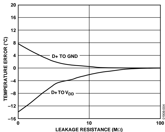
Figure 4. Temperature Error vs. Leakage Resistance
