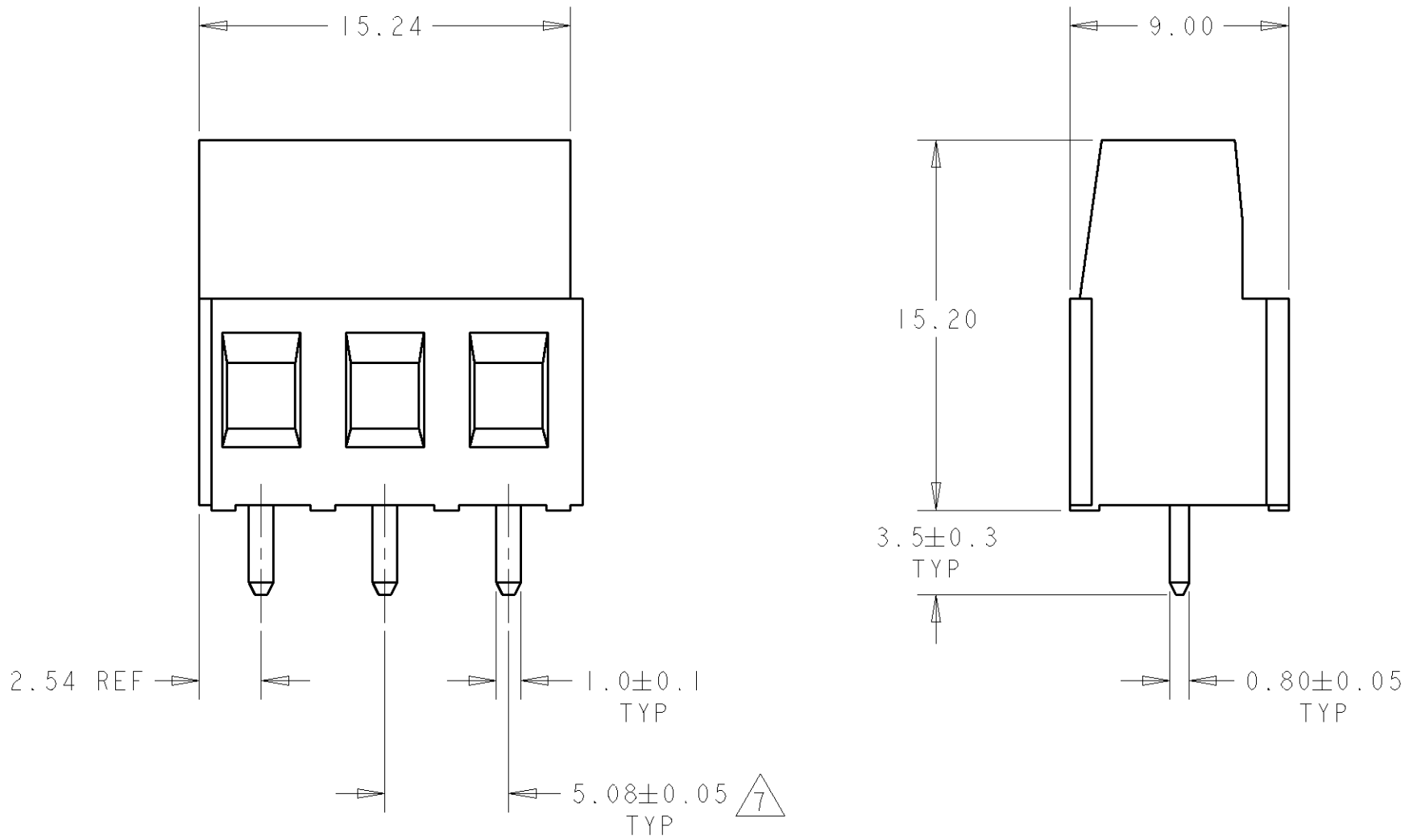
282841-3 AS SHOWN
