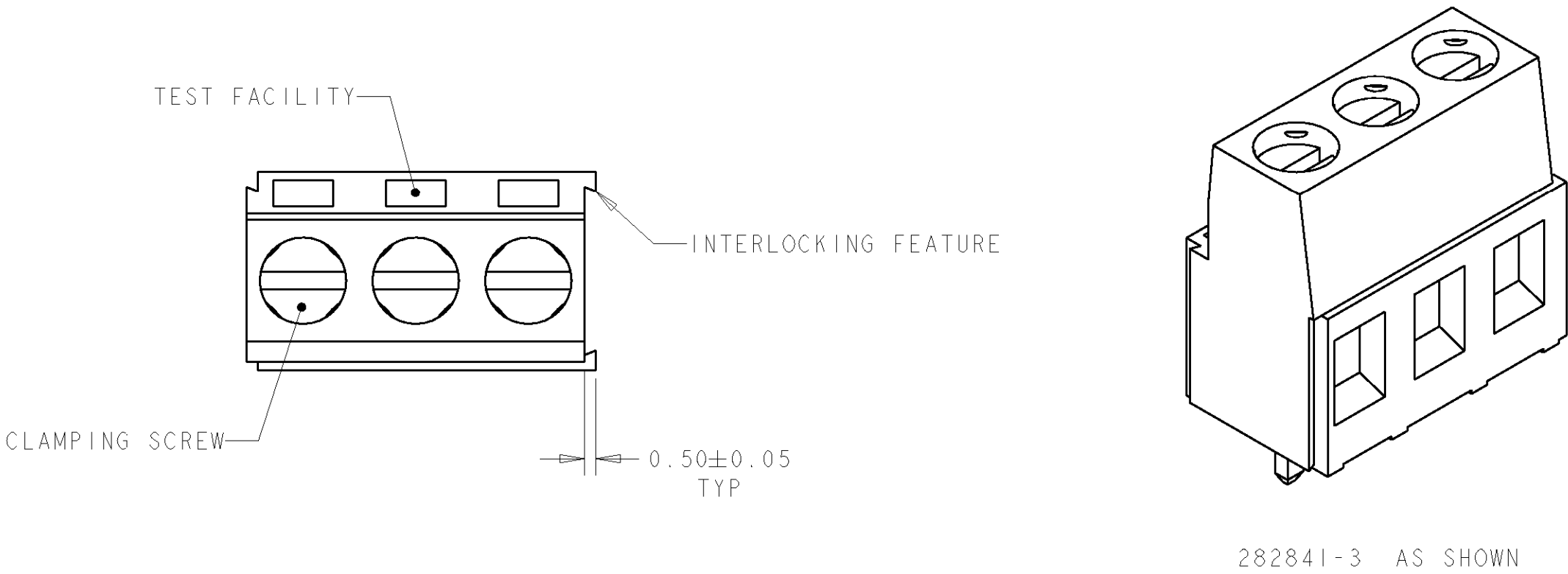
282841-3 AS SHOWN
