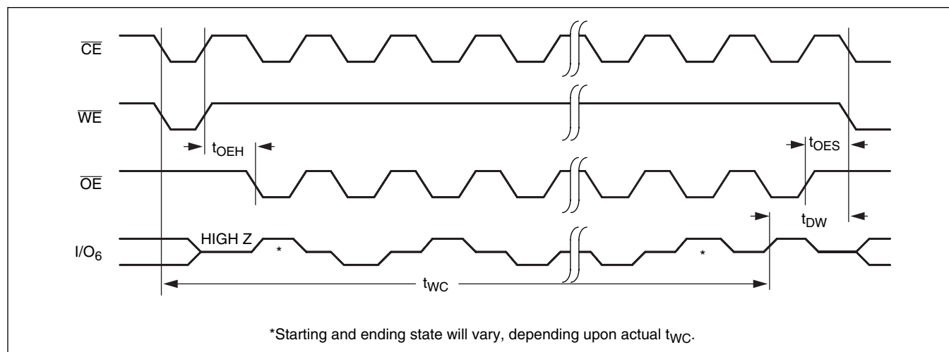
Toggle Bit Timing Diagram
