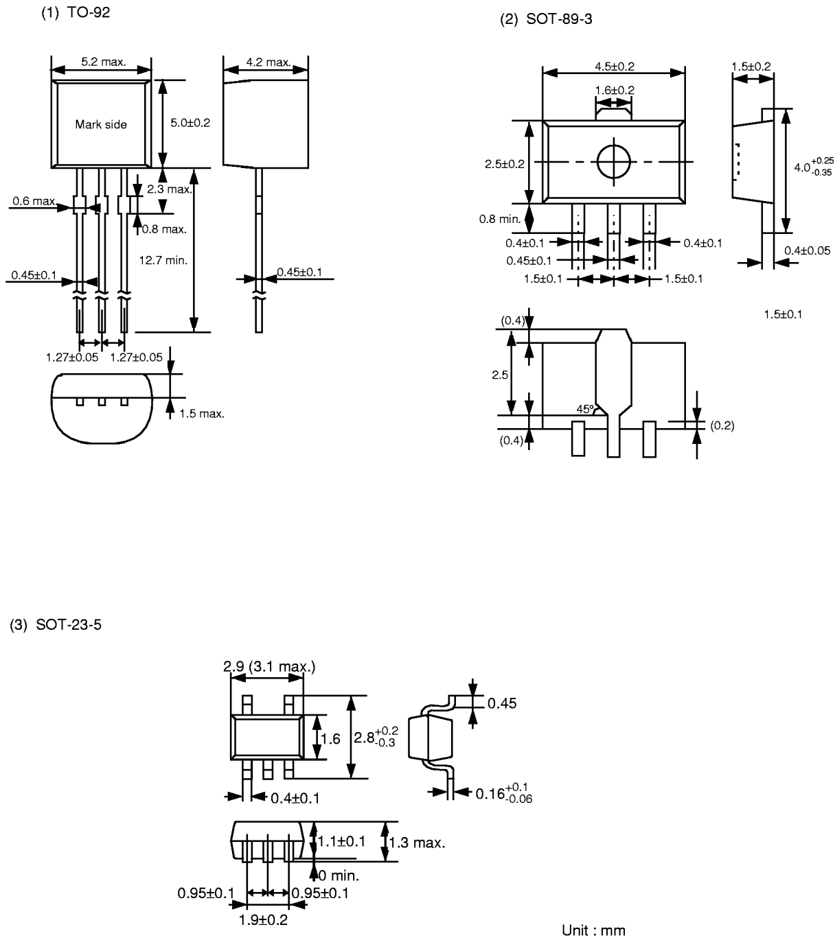
Figure 16 Dimensions
