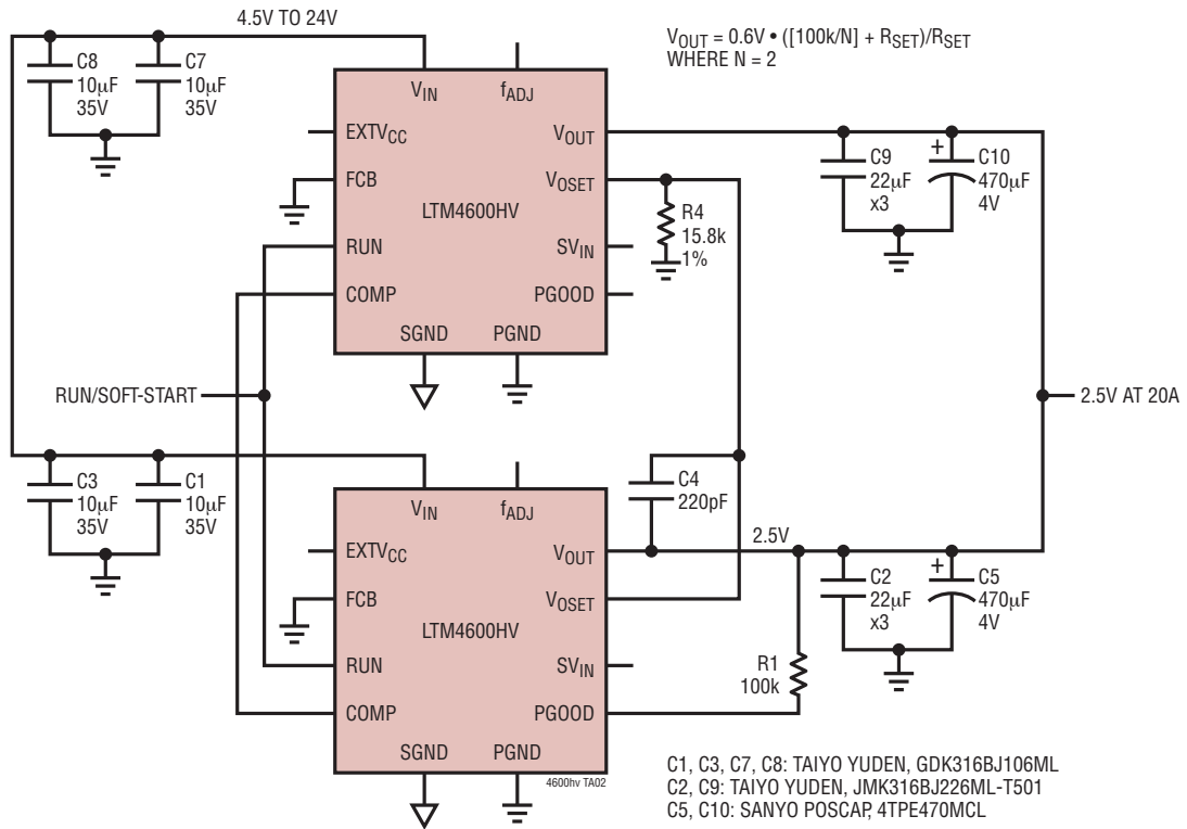
Current Sharing Between Two LTM4600HV Modules
