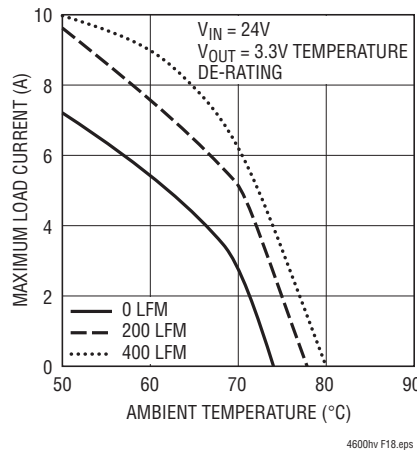
Figure 18. No Heatsink
