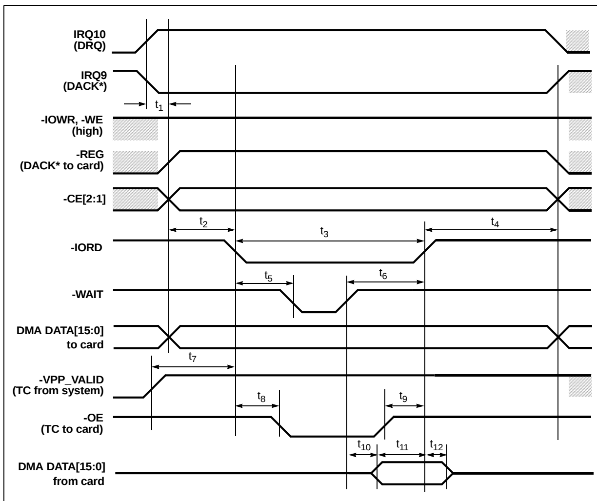
Figure 29. DMA Write Cycle Timing
