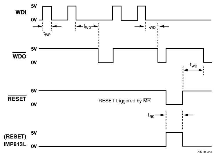
Figure 2. Watchdog Timing
