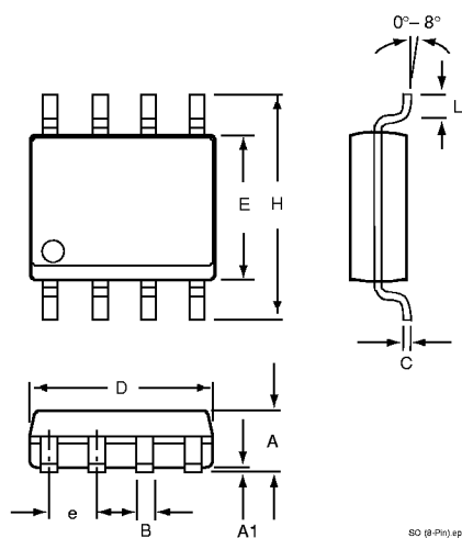
SO (8-Pin).eps
