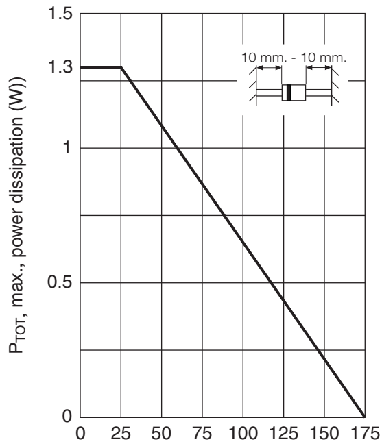
MAXIMUM CONTINUOUS POWER DISSIPATION
