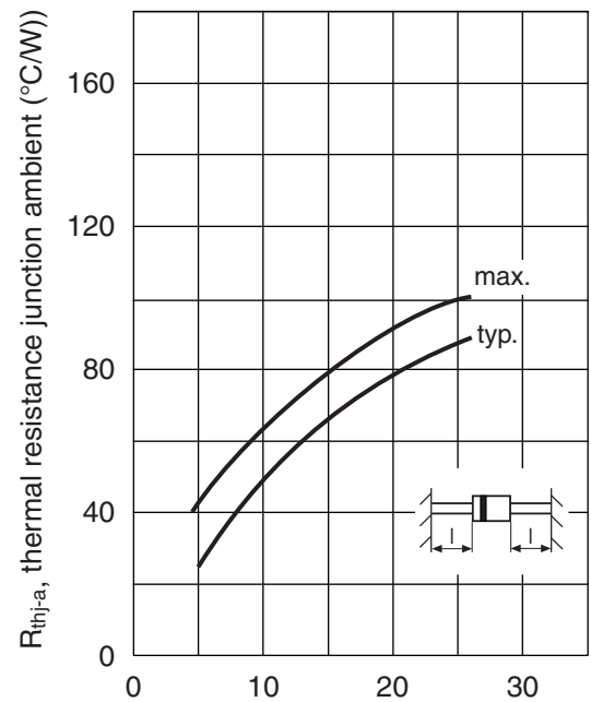
THERMAL RESISTANCE
