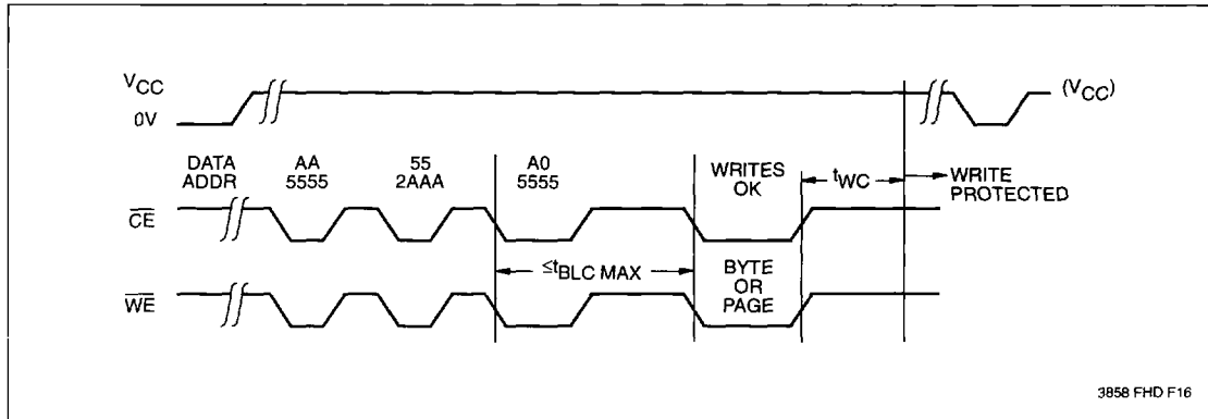
Figure 7. Write Sequence for Software Data Protection
