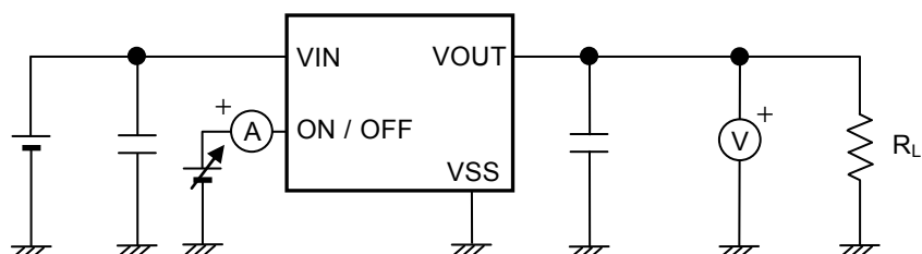
Figure 13 Test Circuit 4
