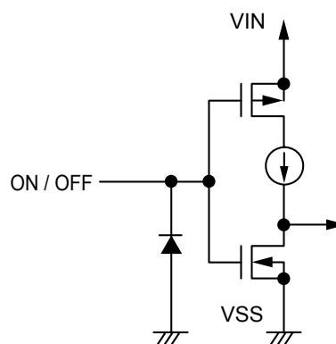
Figure 19 S-1313 Series B / D types
