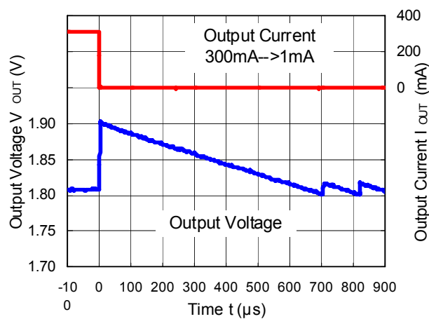
RP505K001C ( V_{IN}=3.6V , V_{OUT}=1.8V ) MODE="L" PWM/VFM automatic shift
