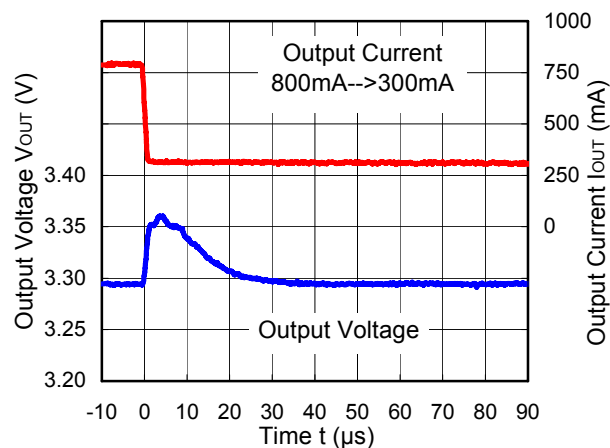
RP505K331A/B ( V_{IN}=5.0V )
