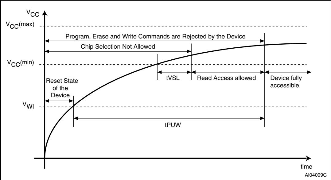
Figure 18. Power-up timing
