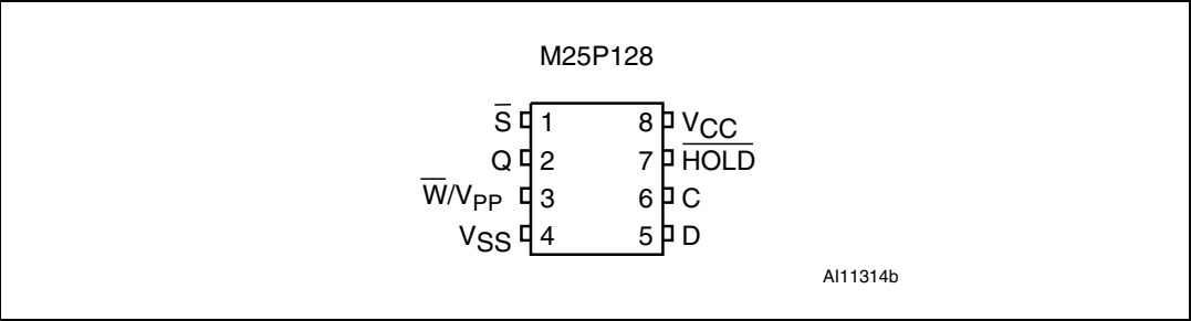
Figure 2. VDFPN connections
