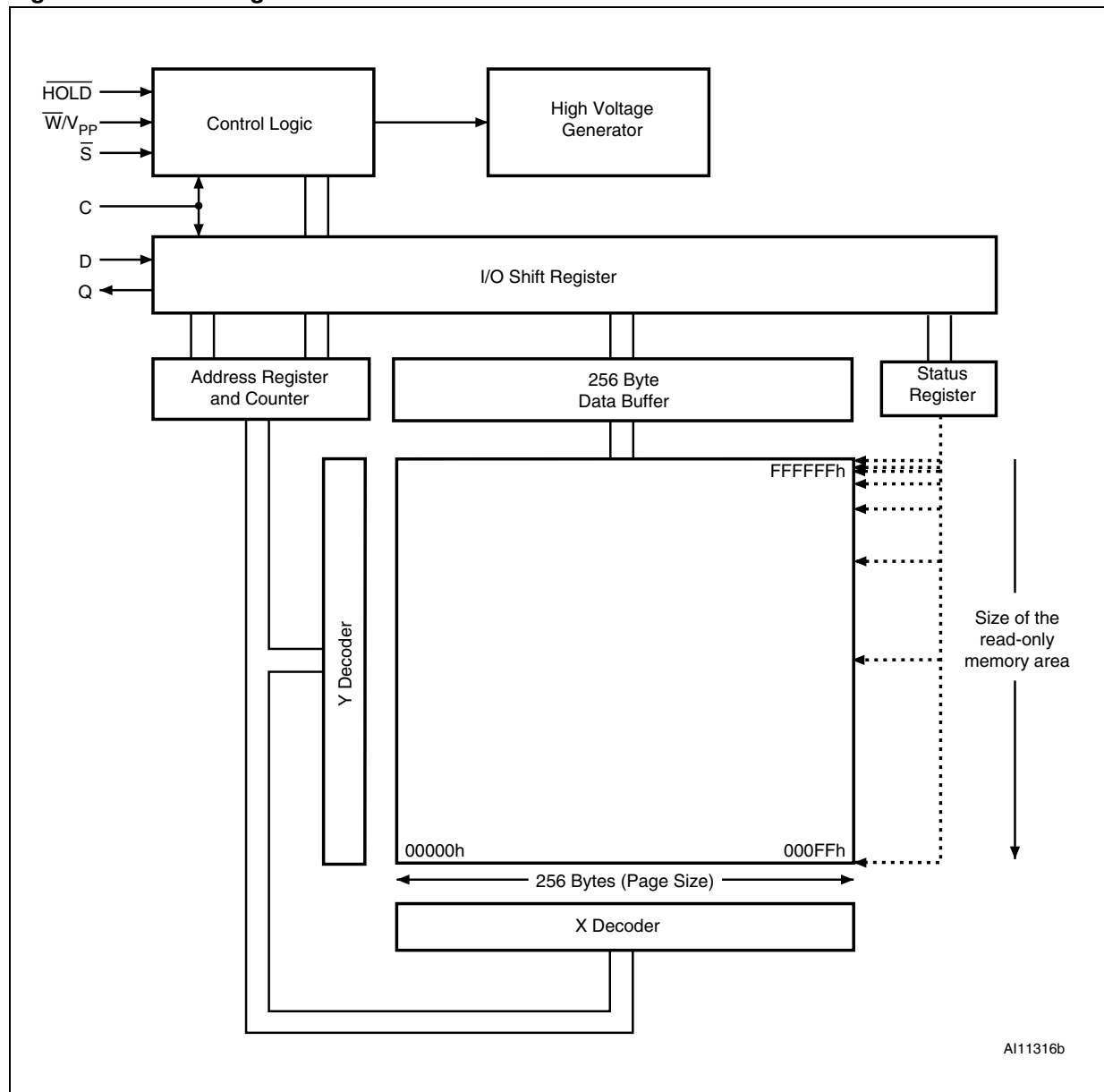
Figure 7. Block diagram
