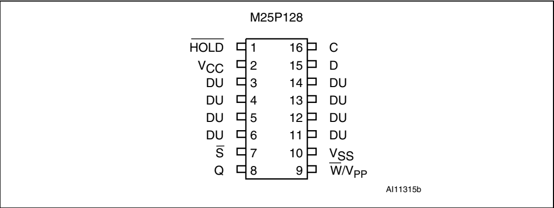
Figure 3. SO connections
