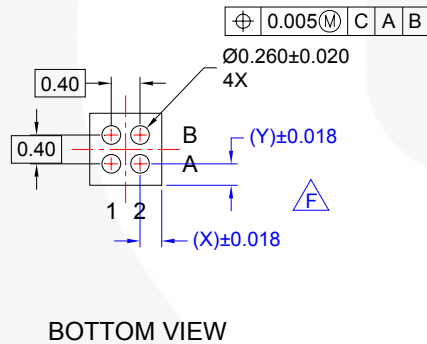
Figure 26. 4 Ball, 0.76 x 0.76 mm Wafer-Level Chip-Scale WLCSP Packaging
