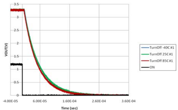
Figure 23. Turn-Off Response (FPF1205 = No Output Pull-Down Resistor) (V IN =3.3V, C IN =1μF, C OUT =0.1μF, R L =500Ω)
