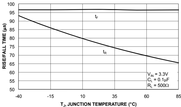
Figure 19. V OUT Rise and Fall Time vs. Temperature at R L =500Ω
