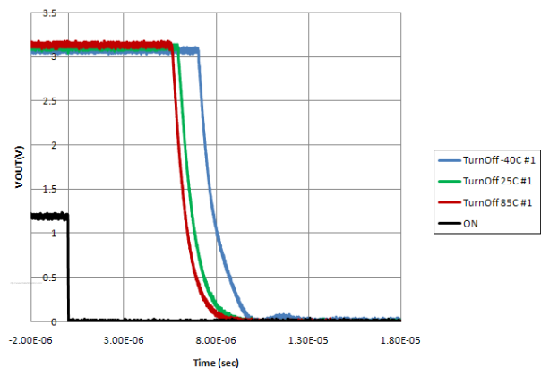
Figure 22. Turn-Off Response (V IN =3.3V, C IN =1μF, C OUT =0.1μF, R L =10Ω)
