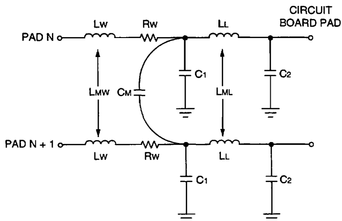
Figure 41. Package Parasitics
