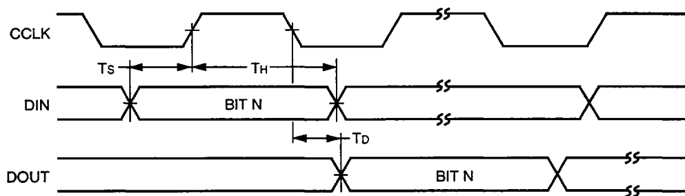
Figure 47. Master Serial Configuration Mode Timing Diagram
