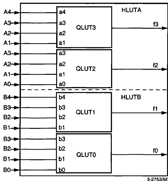
Figure 4. F4 Mode—Four Functions of Four Input Variables
