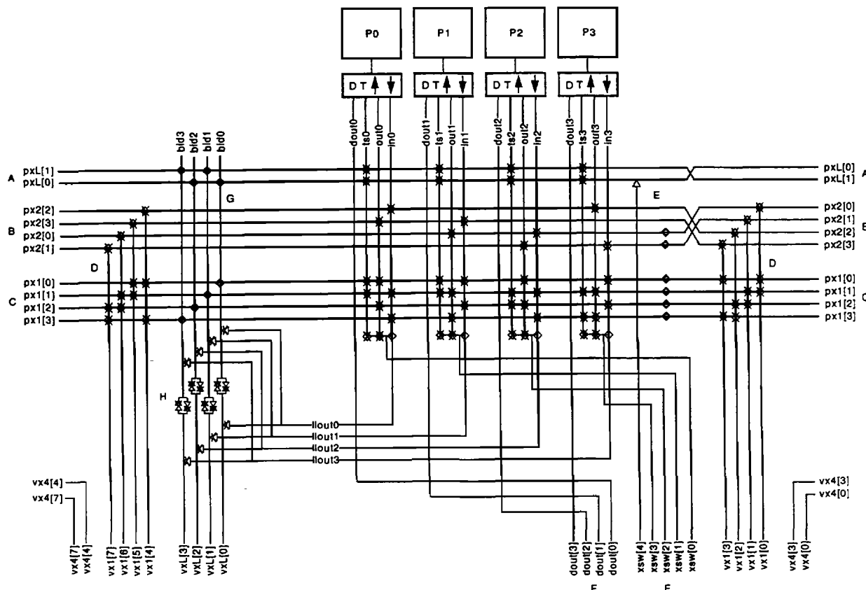
Figure 21. PIC Architecture
