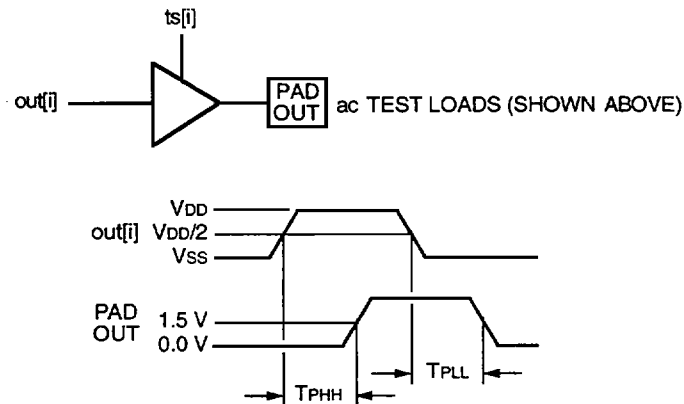
Figure 56. Output Buffer Delays
