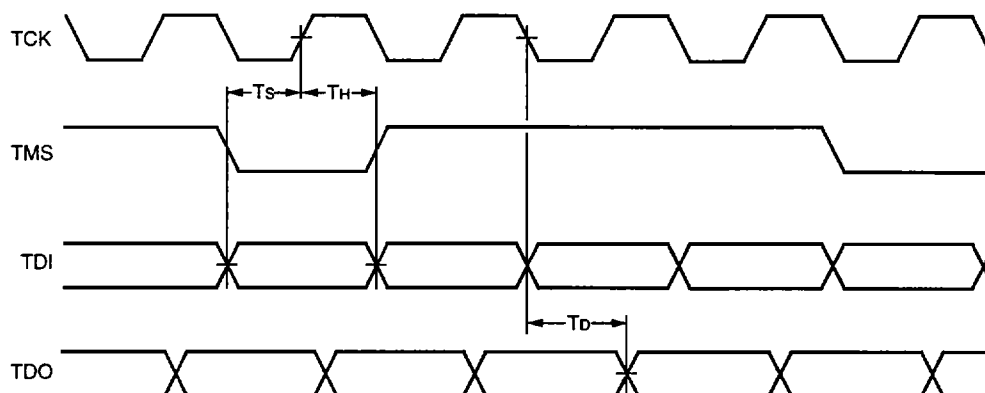
Figure 54. Boundary-Scan Timing Diagram
