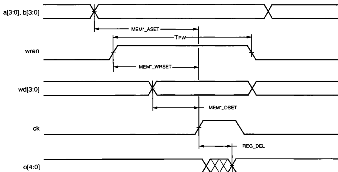
Figure 45. Read During Write—Clocking Data into Flip-Flop
