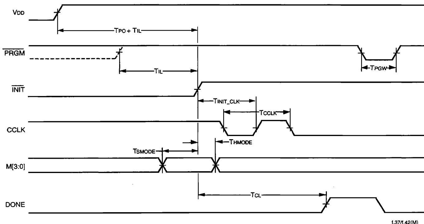
Figure 46. General Configuration Mode Timing Diagram
