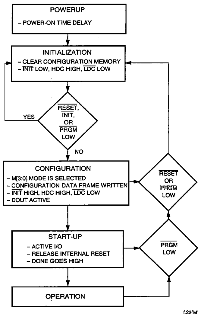
Figure 23. FPGA States of Operation
