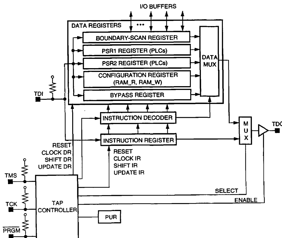
Figure 37. ORCA Series Boundary-Scan Circuitry Functional Diagram
