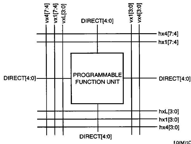
Figure 15. Single PLC View of Inter-PLC R-Nodes
