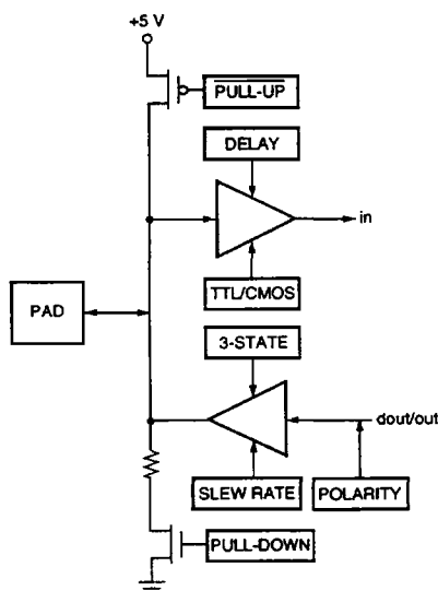
Figure 19. Simplified Diagram of Programmable I/O Cell
