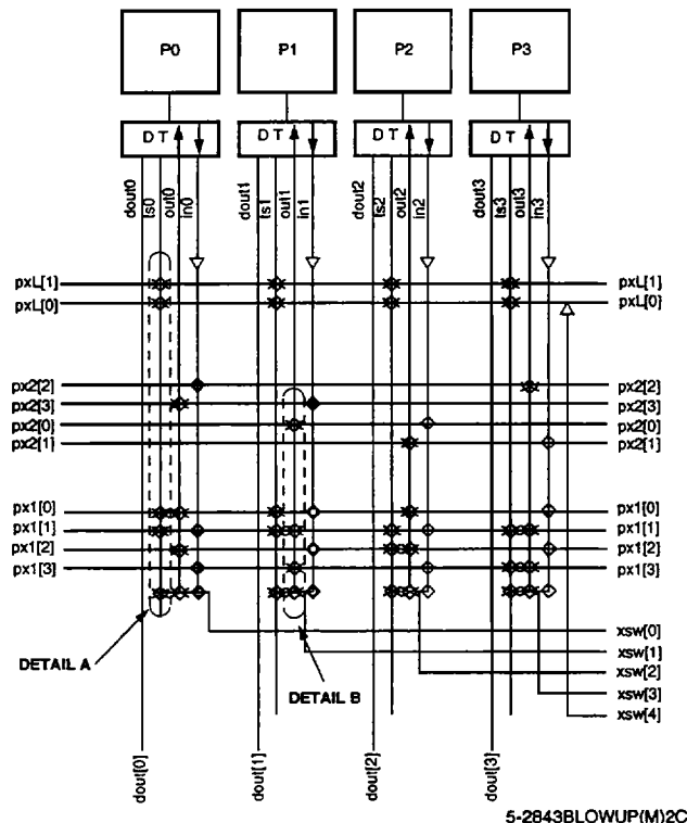
Figure 22. PIC Detail
