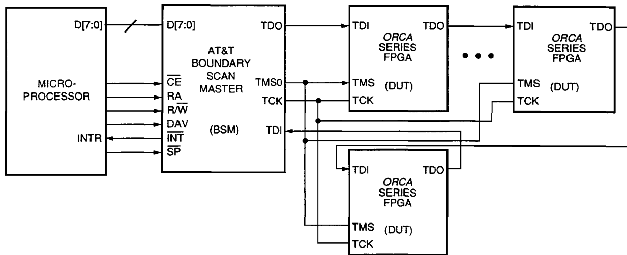
Figure 36. Boundary-Scan Interface
