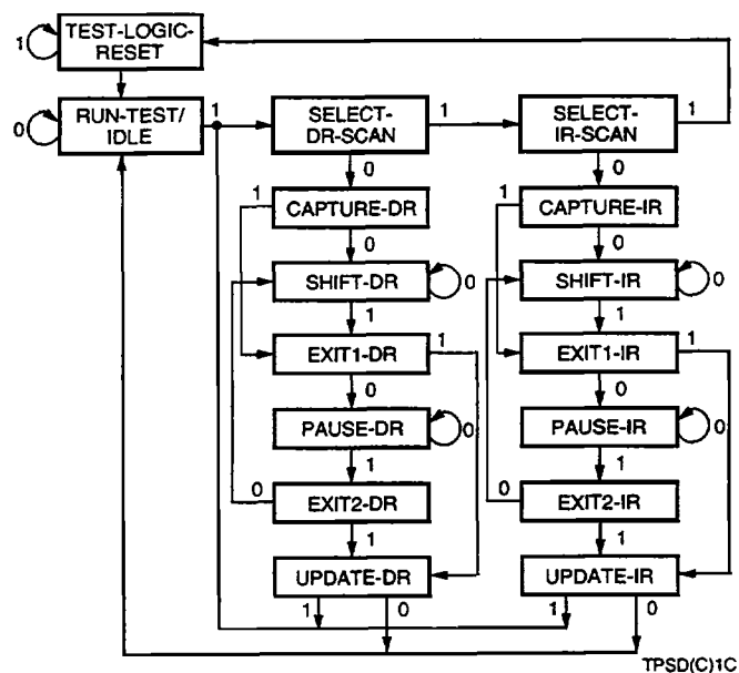
Figure 38. TAP Controller State Transition Diagram
