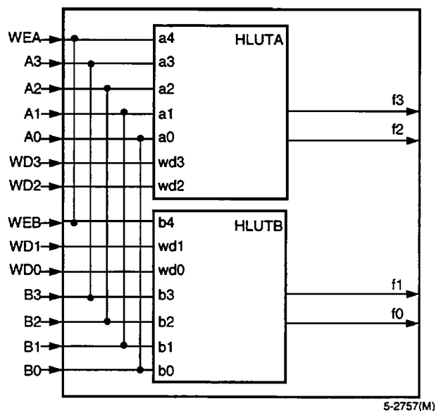
Figure 10. MA/MB Mode— 16 \times 4 RAM
