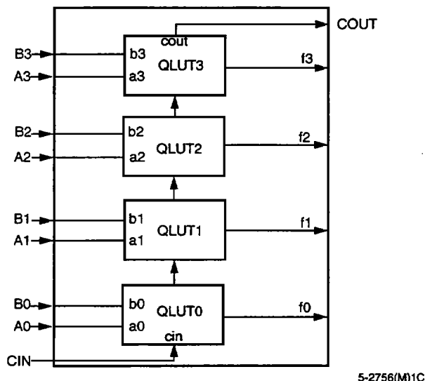
Figure 9. Ripple Mode
