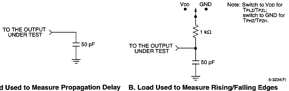
Figure 55. ac Test Loads
