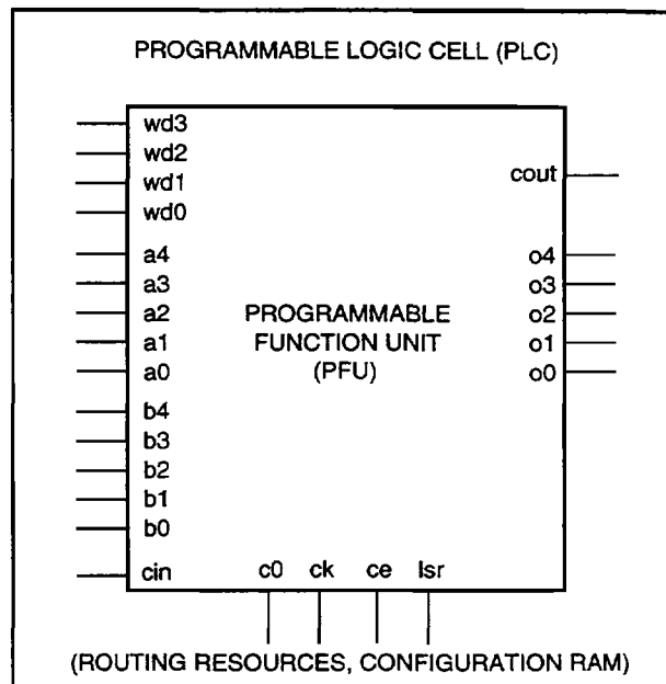
Figure 2. PFU Ports
