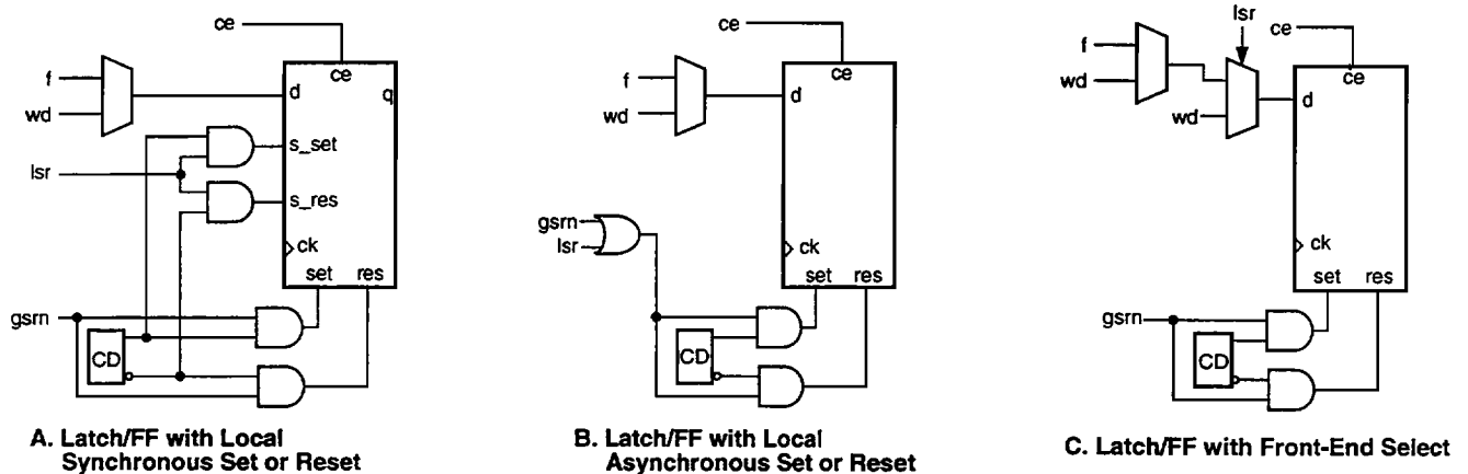
Figure 12. Latch/FF Set/Reset Configurations
