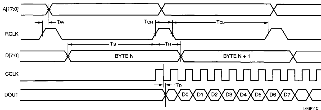
Figure 48. Master Parallel Configuration Mode Timing Diagram
