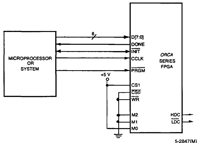
Figure 33. Slave Parallel Configuration Schematic
