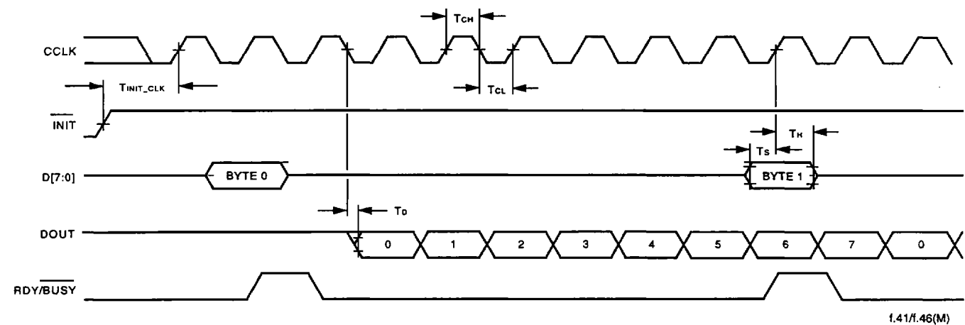
Figure 50. Synchronous Peripheral Configuration Mode Timing Diagram
