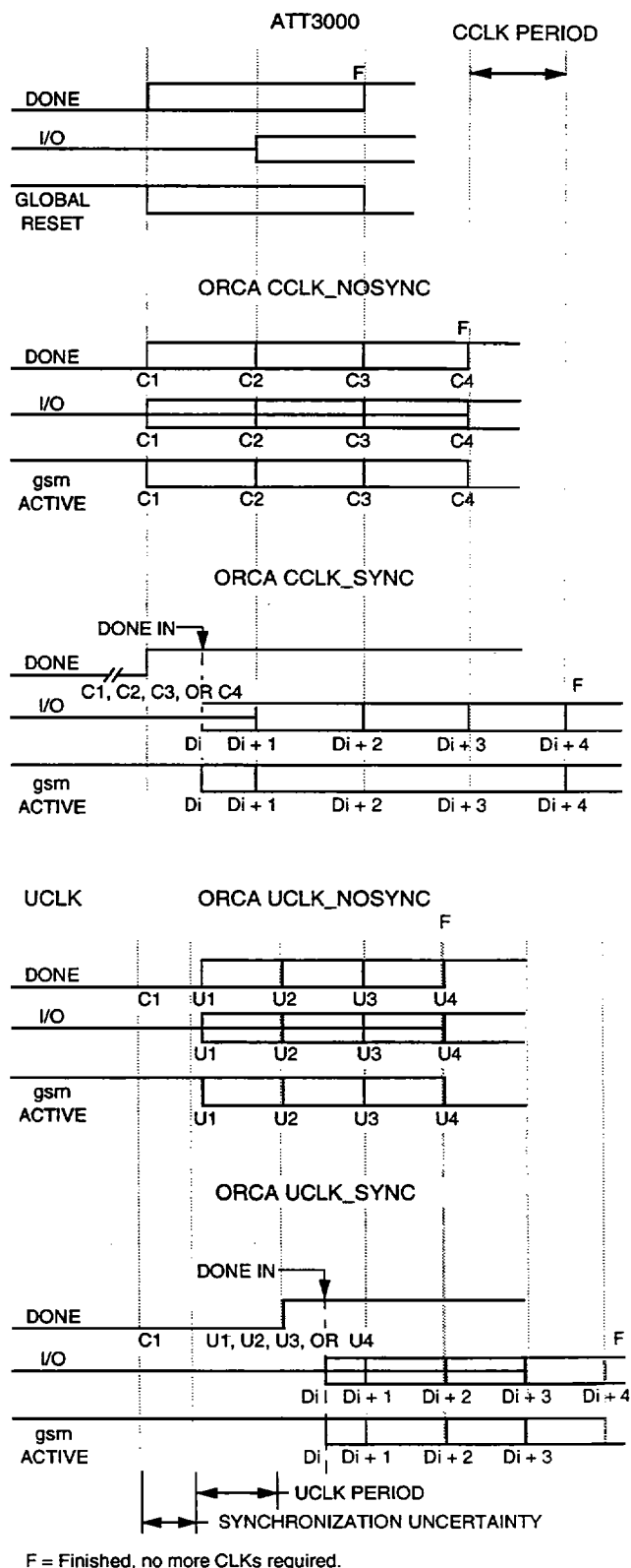
Figure 25. Start-Up Waveform
