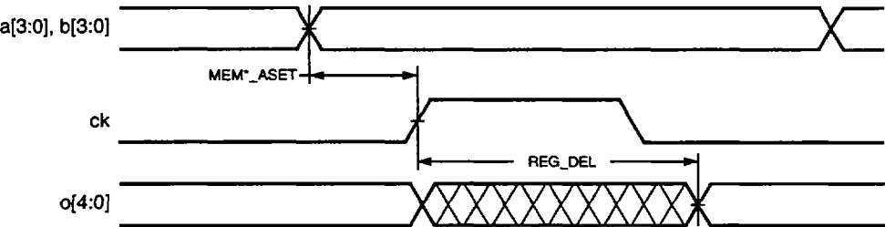
Figure 42. Read Operation—LUT Memory Loading Flip-Flops
