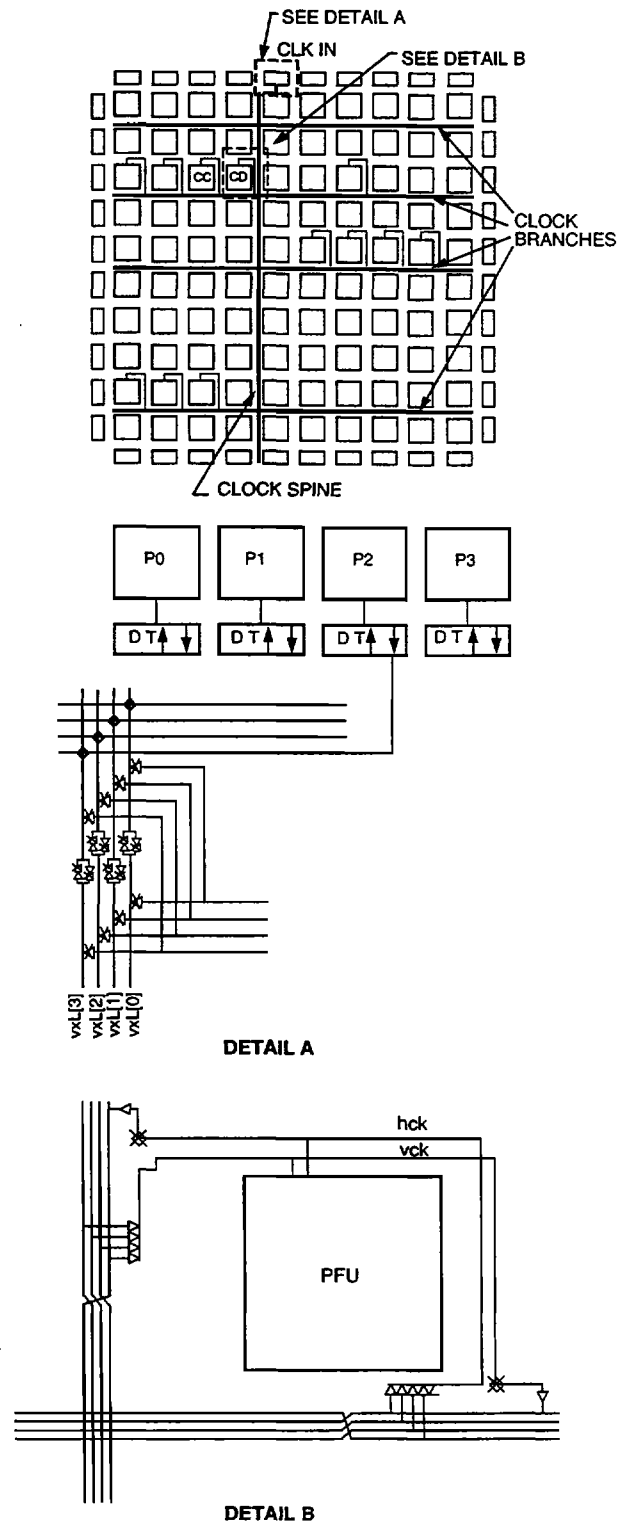
Figure 17. Clock Distribution Network
