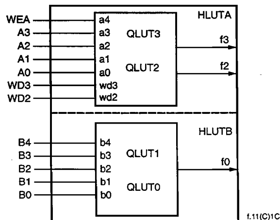
Figure 11. MA/F5 Mode— 16 \times 2 Memory and One Function of Five Input Variables
