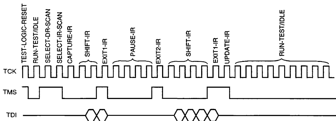
Figure 40. Instruction Register Scan Timing Diagram
