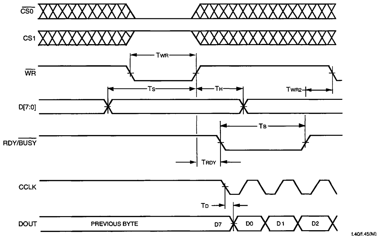
Figure 49. Asynchronous Peripheral Configuration Mode Timing Diagram
