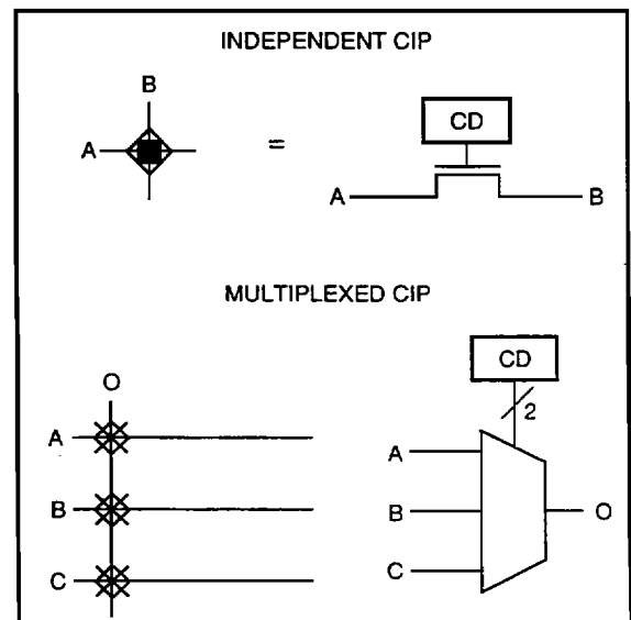
Figure 13. Configurable Interconnect Points
