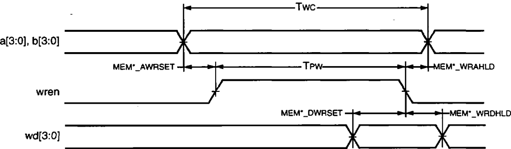
Figure 43. Write Operation
