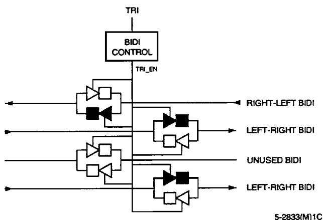
Figure 14. 3-Statable Bidirectional Buffers
