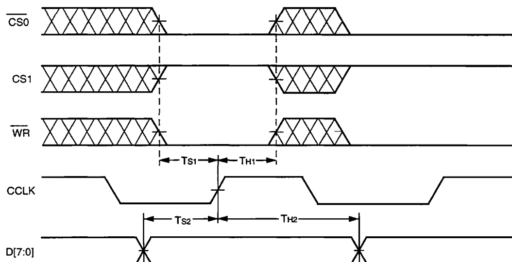
Figure 52. Slave Parallel Configuration Mode Timing Diagram
