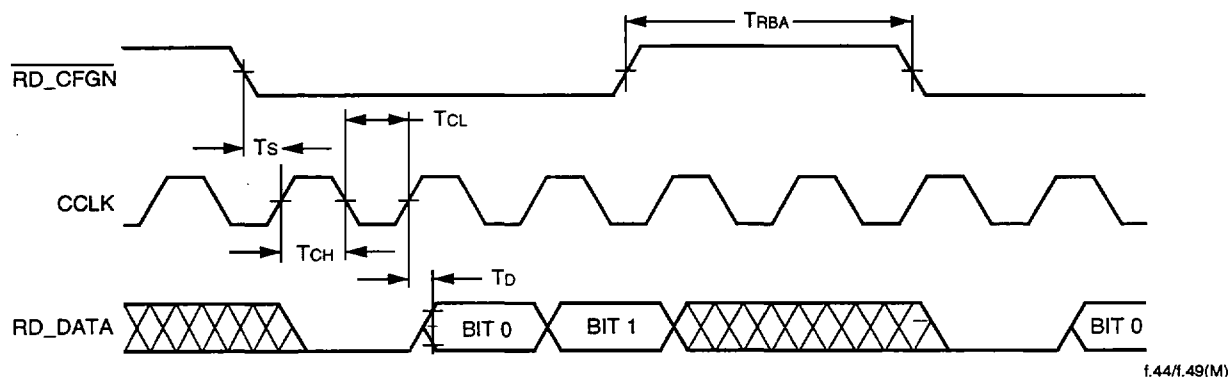
Figure 53. Readback Timing Diagram
