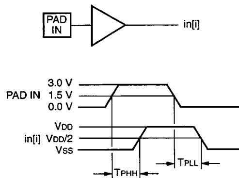
Figure 57. Input Buffer Delays
