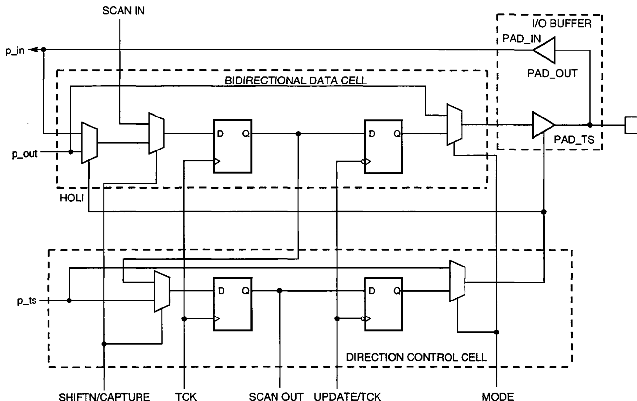
Figure 39. Boundary-Scan Cell
