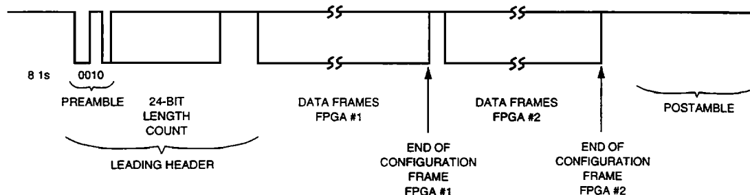
Figure 26. Serial Configuration Data Format
