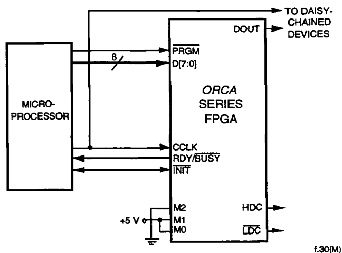
Figure 31. Synchronous Peripheral Configuration Schematic
