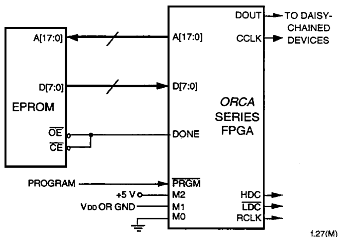
Figure 28. Master Parallel Configuration Schematic
