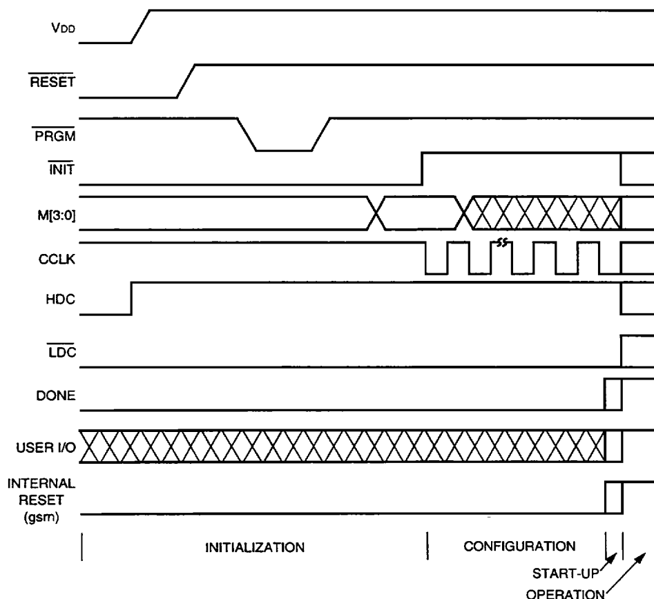
Figure 24. Initialization/Configuration/Start-Up Waveform
