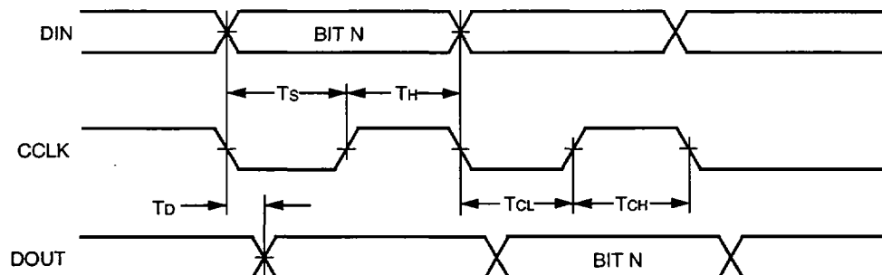
Figure 51. Slave Serial Configuration Mode Timing Diagram
