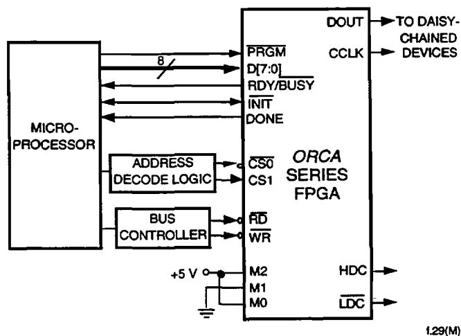
Figure 30. Asynchronous Peripheral Configuration Schematic
