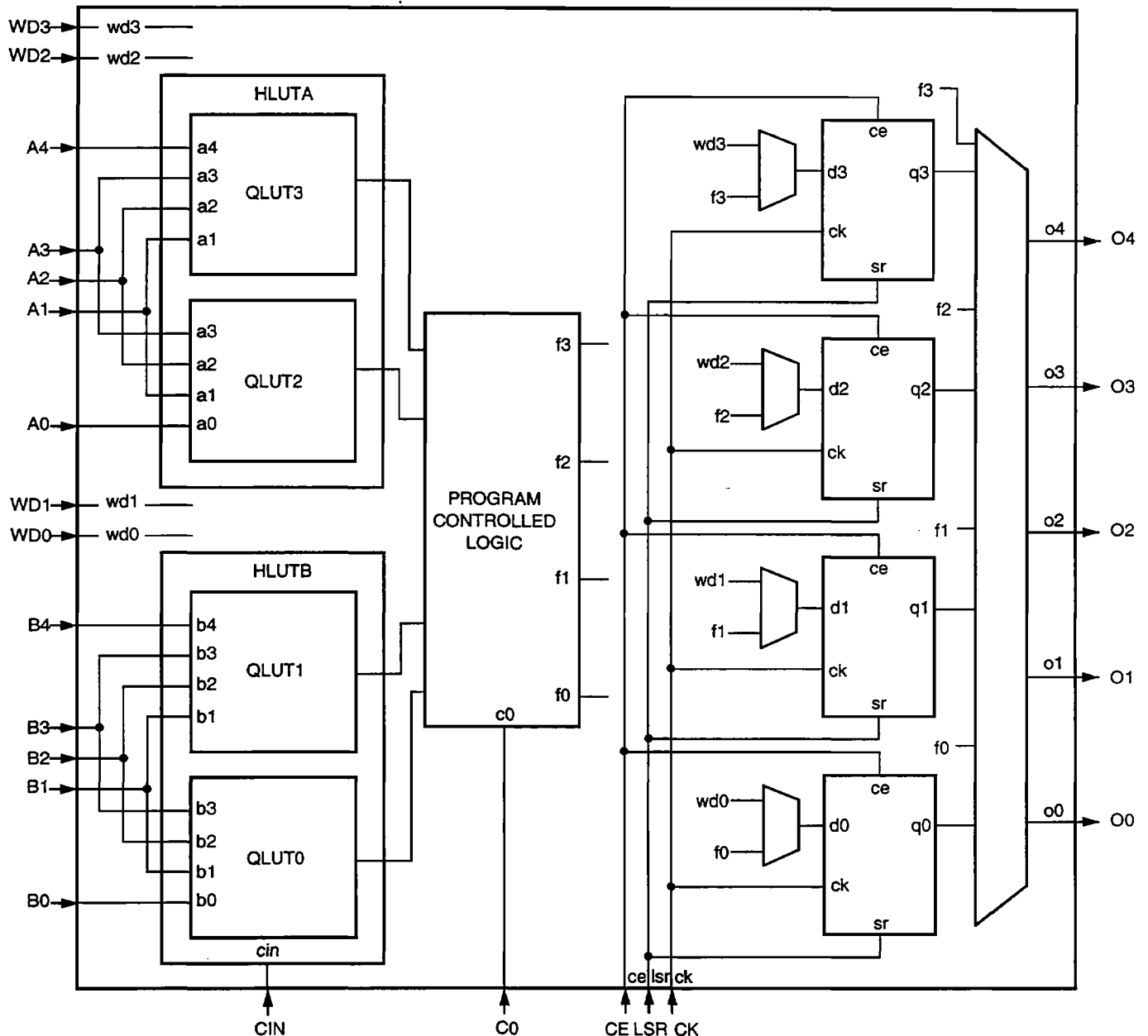
Figure 3. Simplified PFU Diagram
