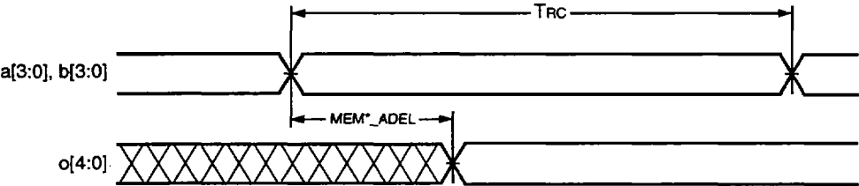
Figure 41. Read Operation—Flip-Flop Bypass
