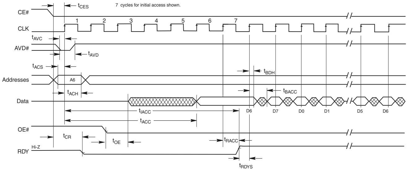
Figure I8. Synchronous Burst Mode Read
