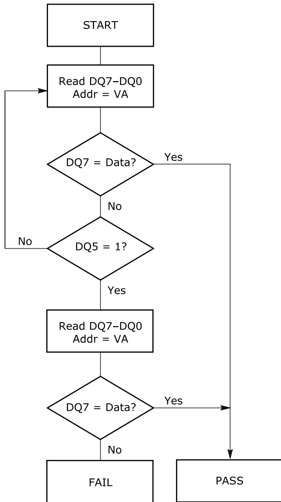
Figure 8. Data# Polling Algorithm
