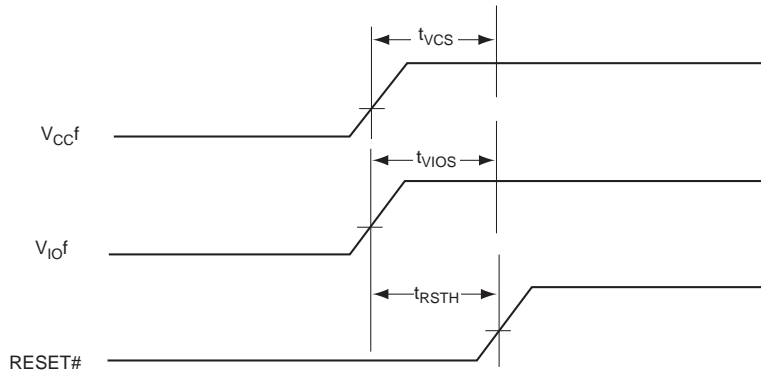
Figure I4. V CC Power-up Diagram
