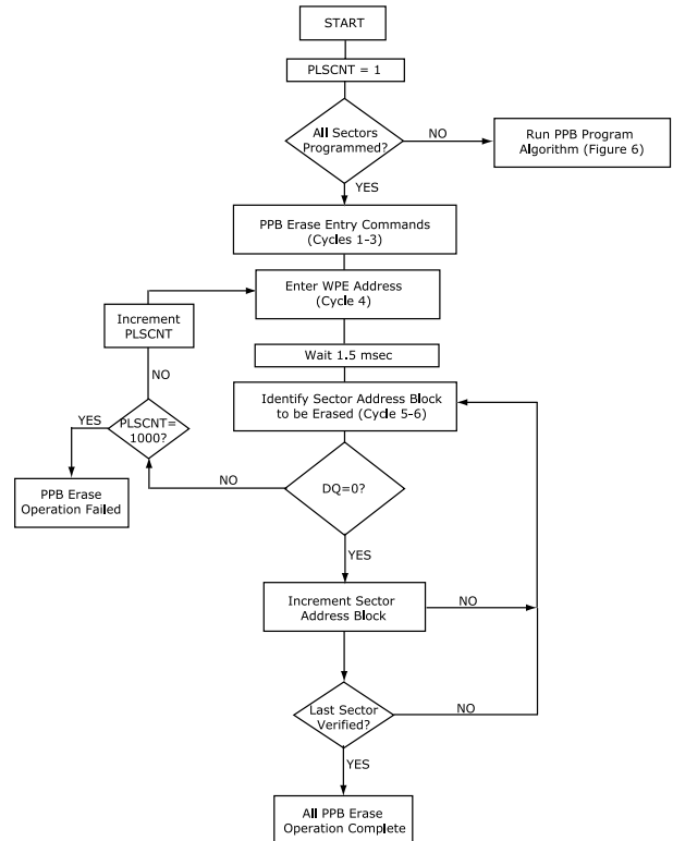
Figure 7. All PPB Erase Algorithm
