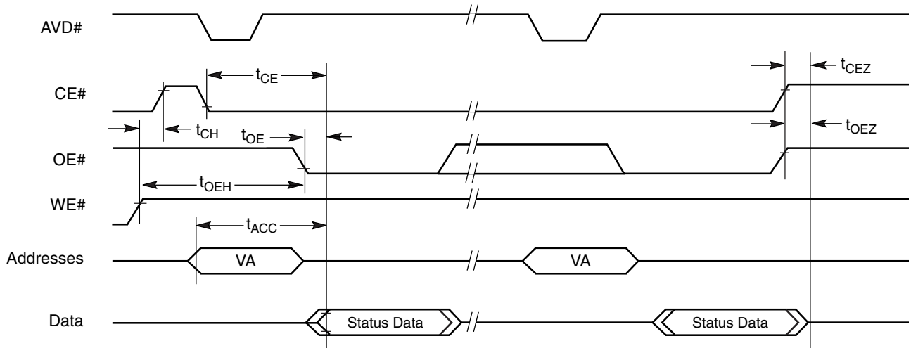
Figure 40. Data# Polling Timings (During Embedded Algorithm)
