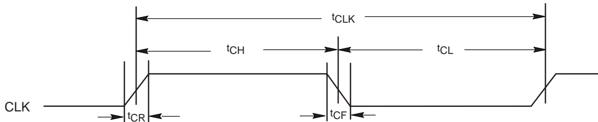
Figure I5. CLK Characterization
