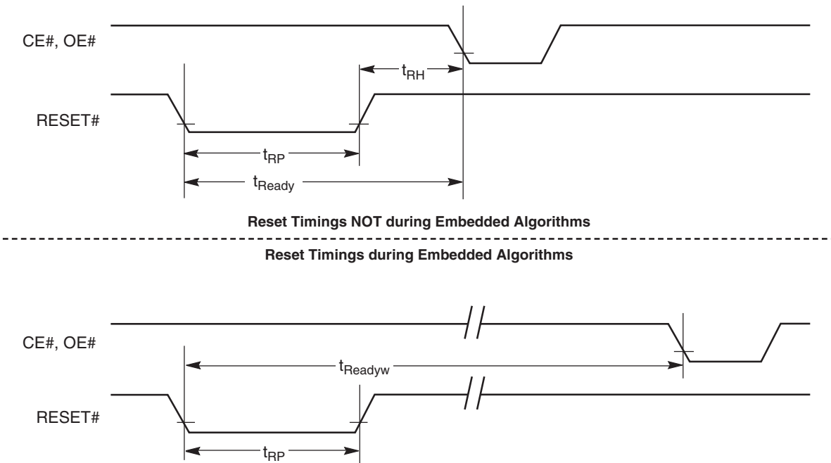
Figure 33. Reset Timings
