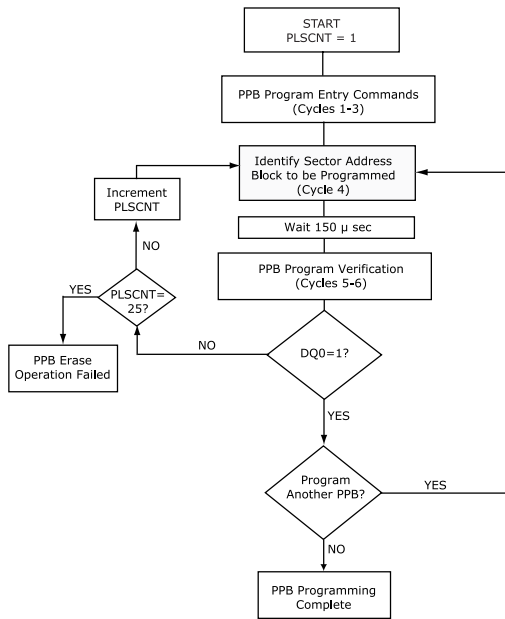
Figure 6. PPB Program Algorithm
