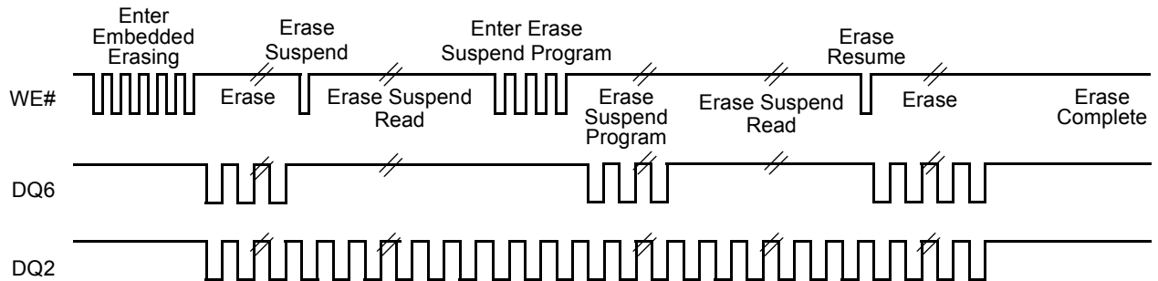
Figure 42. Synchronous Data Polling Timings/Toggle Bit Timings
