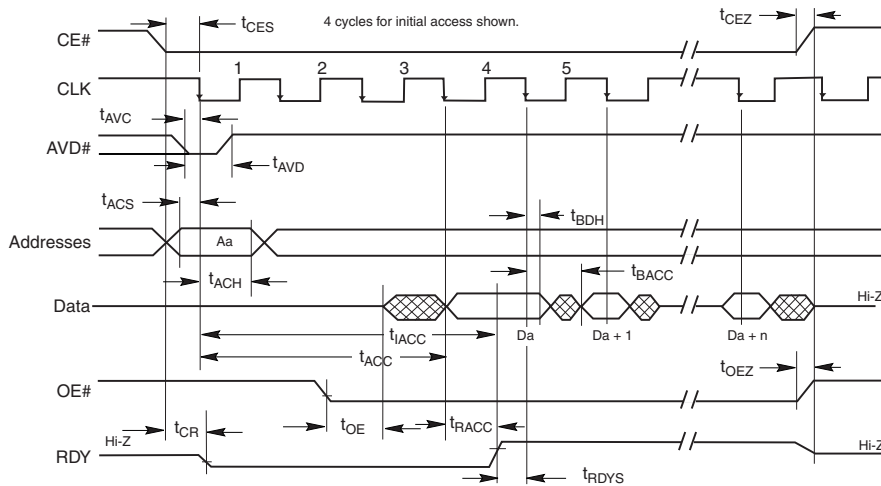
Figure 16. CLK Synchronous Burst Mode Read (Rising Active CLK)
