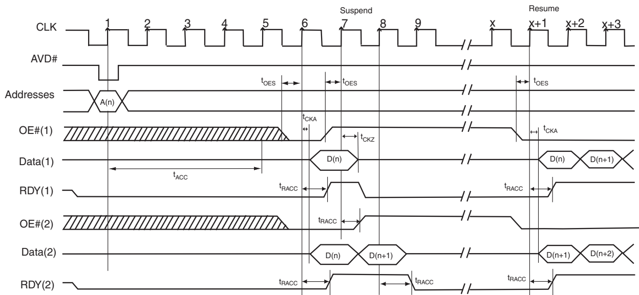
Figure 25. Standard Handshake Burst Suspend prior to Initial Access
