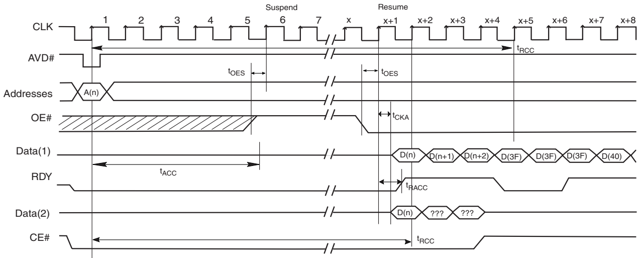
Figure 29. Standard Handshake Burst Suspend at address 3Eh/3Fh (with I Access CLK)
