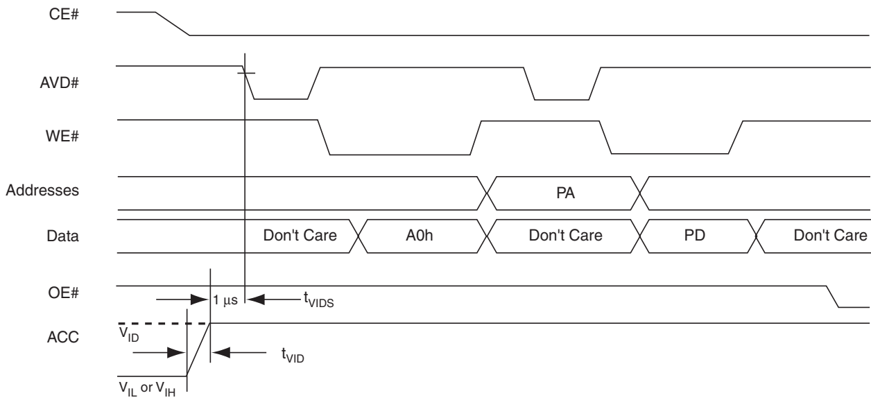
Figure 39. Accelerated Unlock Bypass Programming Timing
