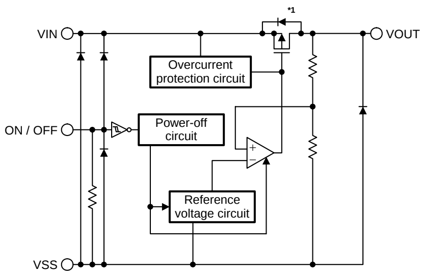
*1. Parasitic diode
